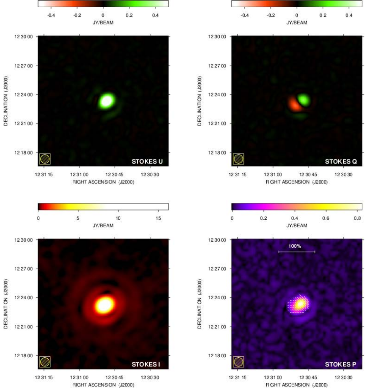
Fig. 6. SRT total intensity and polarization images of Virgo A with SARDARA resulting from the spectral average of the bandwidth between 18 GHz and 20 GHz, see text. The top-left and top-right panels show the images of Stokes parameters U and Q, respectively. The bottom-left panel shows the total intensity image. The bottom-right panel shows the polarization intensity P = \sqrt{U^2 + Q^2} with the polarization vector over imposed. The length of the vectors is proportional to the fraction polarization while the polarization position angle represents the direction of the E-field (not corrected for the Faraday rotation effect).
