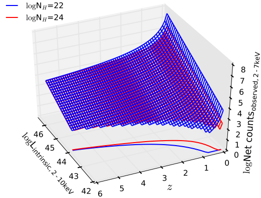
Fig. 24.— Conversion surfaces from any point in the L_X - z space to hard-band observed net counts, obtained at the aimpoint with a \log N_H of 22 (blue grid and line) and 24 (red grid and line). Only the parts above 80 net counts of the surfaces are shown. The lines in the L_X - z space at the base are projections of the intersections of the two surfaces with the plane where net counts = 80.
