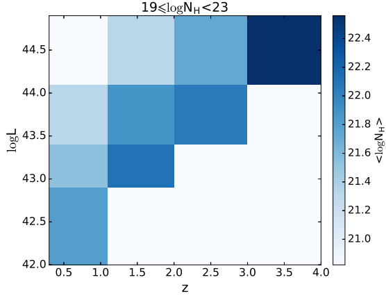
Fig. 34.— Mean \log N_H in grid, combining CDF-S and C-COSMOS data. Only values below 23 are considered. Values below 19 are taken as 19. White cells are excluded.
