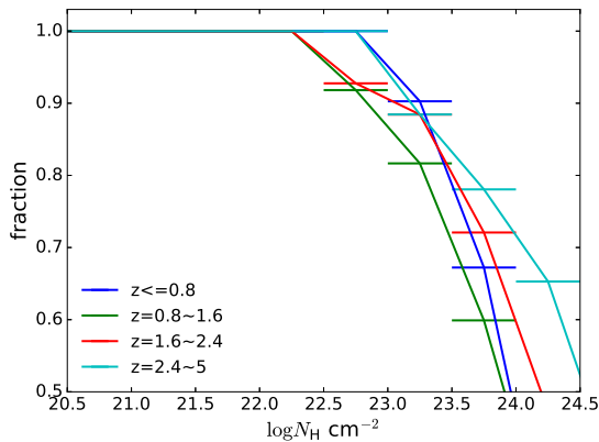
Fig. 29.— The fraction of sources detectable within our sample with a given N_H , computed for the luminosity range \log L within 42–45, in four redshift bins.
