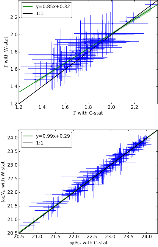
Fig. 16.— Power-law slope and column density as obtained using spectral fitting method C (standard C statistic) and D ( W statistic). The best-fit lines and 1\sigma confidence intervals are plotted with the green lines and green shadings.
