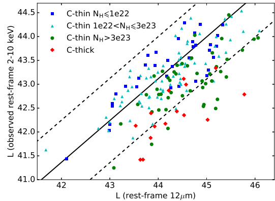
Fig. 7.— Scatter plot of the rest-frame 2–10 keV observed X-ray luminosity and the total rest-frame 12\mu\text{m} luminosity. The sources are divided into four subsamples according to the N_H . The solid line corresponds to the best-fit L_{2-10 \text{ keV, intrinsic}} - \log L_{12\mu\text{m}} correlation, and the dashed lines represent its 2\sigma scatter.
