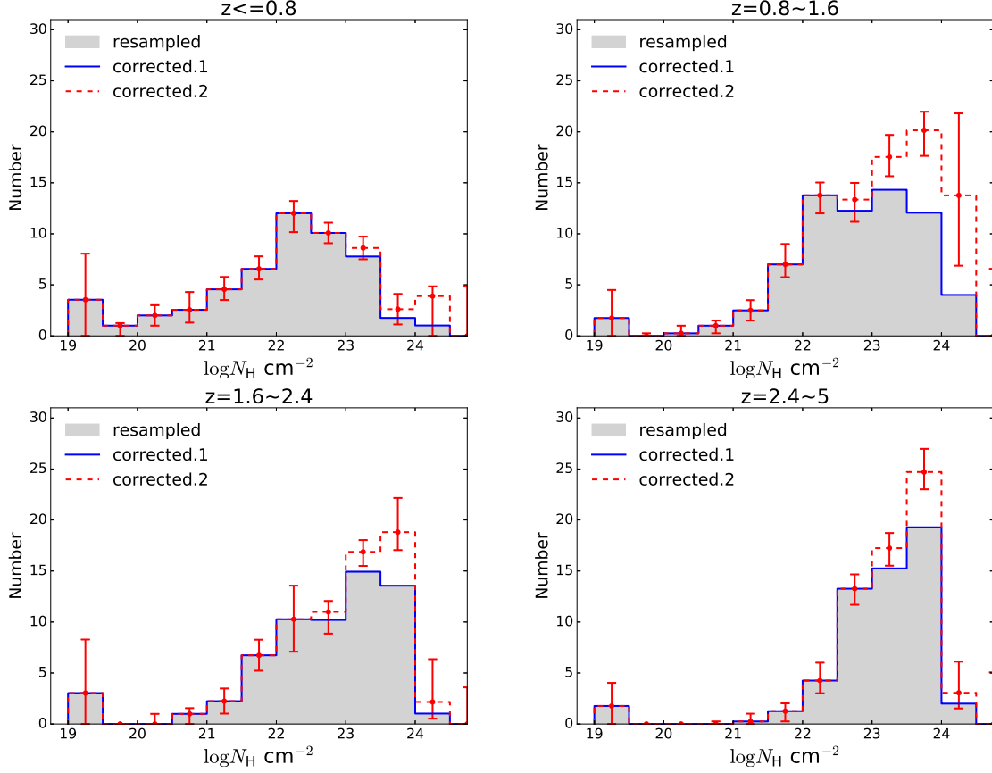
Fig. 27.— N_H distributions in the observable spaces corresponding to four redshift bins, as show in Figure 25. The 90% percentile luminosity range of the sources in the four redshift bins are 41.65~43.40, 42.57~44.12, 43.05~44.35, 43.46~44.76, respectively, in the order of arising z . Grey filled histograms show the resampled N_H distribution of the Compton-thin sources, the same as plotted in Figure 12. The “corrected.1” (blue solid line) histogram shows the N_H distribution after correction for the inhomogeneous survey depth, which has a minor effect. Then after further correcting for the N_H -dependent Malmquist bias, the N_H distribution is plotted as the “corrected.2” (red dashed line) histogram. The 1\sigma error obtained from bootstrapping is plotted on the “corrected.2” histogram.
