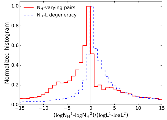
Fig. 11.— Resampled k distributions, calculated between each pair of N_H variable spectra (red) and each pair of random values of the same spectrum (blue). The histograms are normalized to the peak value.
