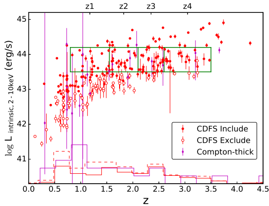
Fig. 31.— Scatter plot of the AGN sample in the luminosity – redshift space, with 90% errors on luminosity. The \log N_H < 24 N_H -complete subsample is plotted with red solid points (marked as “Include”) and the other Compton-thin sources with red empty points (marked as “Exclude”). At the bottom, the normalized redshift distributions of the complete subsample (“Include”) and the whole sample (“Include”+“Exclude”) are shown as red solid and dashed histograms, respectively. The Compton-thick sources are also shown with the magenta points and blue histogram. The four green boxes, which are marked as z1 , z2 , z3 , and z4 , are the regions selected to analyze the N_H dependence on redshift. Empty points are excluded from this analysis even if they fall in the selected bins.
