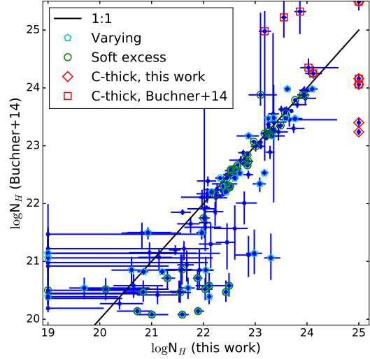
Fig. 22.— Column densities N_H with 1\sigma errors measured in Buchner et al. (2014) and in this work. Sources identified as Compton-thick in Buchner et al. (2014) and in this work are marked with red squares and red diamonds, respectively. We set the \log N_H of our Compton-thick sources at 25. If N_H is found to vary among different periods in this work, all the values are plotted and marked with cyan pentagons. Sources having soft excess components, whose spectral model contains an additional power-law, are marked with green circles.
