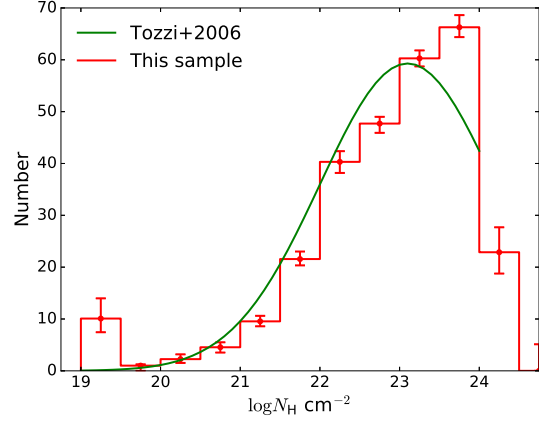
Fig. 30.— Intrinsic N_H distribution of our whole sample, measured by summing up the intrinsic N_H distributions in the four redshift bins ( z < 5 ) as shown in Figure 27. The 90% percentile luminosity range of our sample is 42.41~44.45. The green line which is derived from the 1Ms CDF-S by Tozzi et al. (2006), is a log-normal distribution centered at \log N_H = 23.1 with a \sigma = 1.1 and normalized to the number of AGN used in this work between \log N_H of 19 and 24.
