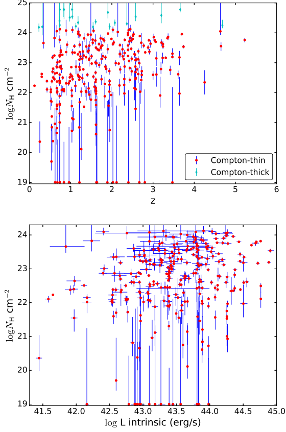
Fig. 15.— Best-fit N_H versus redshift. Error bars correspond to 1\sigma . Some sources with very low or very high N_H have very large uncertainties. Scatter plot of the best-fit N_H and rest-frame 2–10 keV unabsorbed luminosities of the Compton-thin sources. Error bars correspond to 1\sigma .
