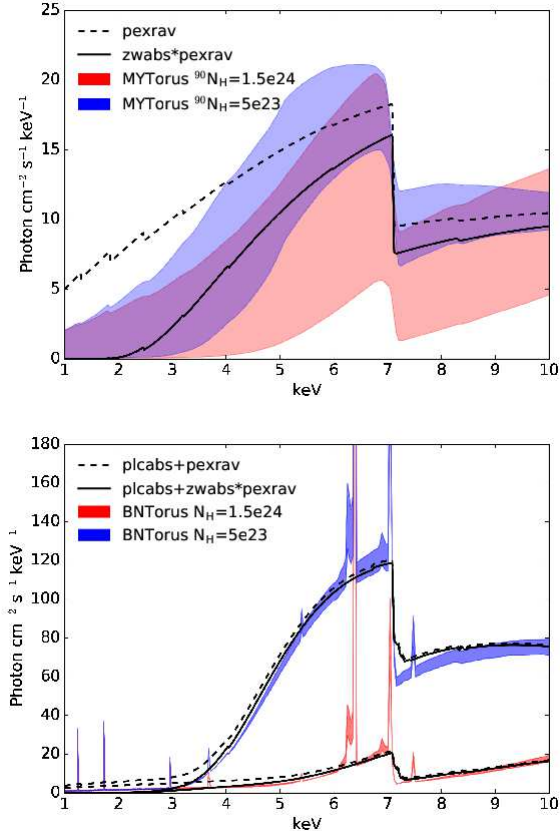
Fig. 6.— Upper panel: the reflection model adopted in this work ( \text{zwabs} \times \text{pexrav} with an ^p N_{\text{H}} of 10^{23} \text{ cm}^{-2} , black solid line) compared with MYTorus reflection models (color filled regions) with diameter column densities of ^90 N_{\text{H}} = 5 \times 10^{23} \text{ cm}^{-2} (blue) and ^90 N_{\text{H}} = 1.5 \times 10^{24} \text{ cm}^{-2} (red) between inclination angles of \theta = 0^\circ (face-on) and \theta = 90^\circ (edge-on). The unabsorbed \text{pexrav} model is plotted with a dashed black line. All the models are derived from the same intrinsic primary power-law and have z = 0 . Lower panel: the model of transmitted power-law plus reflection adopted in this work ( \text{plcabs} + \text{zwabs} \times \text{pexrav} , black solid lines) compared with BNTorus models (color filled regions) in two cases with N_{\text{H}} = 5 \times 10^{23} \text{ cm}^{-2} (blue) and N_{\text{H}} = 1.5 \times 10^{24} \text{ cm}^{-2} (red), respectively. The filled ranges correspond to torus opening angles between \theta_{\text{torus}} = 30^\circ and \theta_{\text{torus}} = 60^\circ . Without the “self-absorption”, the \text{plcabs} + \text{pexrav} model is plotted with black dashed line. All the models have z = 0 . They are all derived from the same intrinsic primary power-law, but the normalizations of the \text{plcabs} -based models are multiplied by factors of 75% and 50% in the cases of N_{\text{H}} = 5 \times 10^{23} \text{ cm}^{-2} and N_{\text{H}} = 1.5 \times 10^{24} \text{ cm}^{-2} , respectively.
