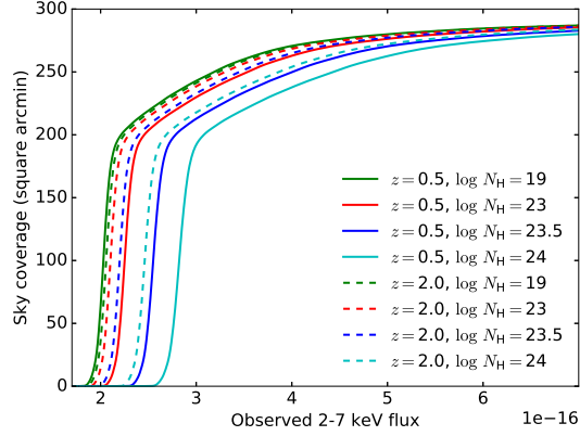
Fig. 23.— The sky coverage as a function of the 2-7 keV observed flux ( \text{erg cm}^{-2} \text{s}^{-1} ) corresponding to 80 hard-band net counts for a set of N_H values at redshifts of 0.5 (solid lines) and 2 (dashed lines).
