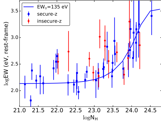
Fig. 10.— Scatter plot of \log N_H and \log EW of the detected narrow Fe K\alpha line. Sources with secure and insecure redshift measurements are plotted in blue and red, respectively. The blue line shows our model of the line with an N_H -independent flux and EW=135 eV when unobscured.
