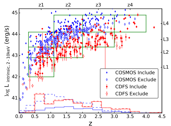
Fig. 33.— Same as Figure 31, but including C-COSMOS data (red for CDF-S, blue for C-COSMOS). The selected subsamples are complete for \log N_H < 23 .
