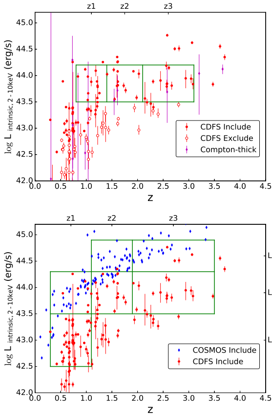
Fig. 35.— The upper and lower panels are the same as Figure 31 and Figure 33 respectively, but only include spectroscopic- z sources.
