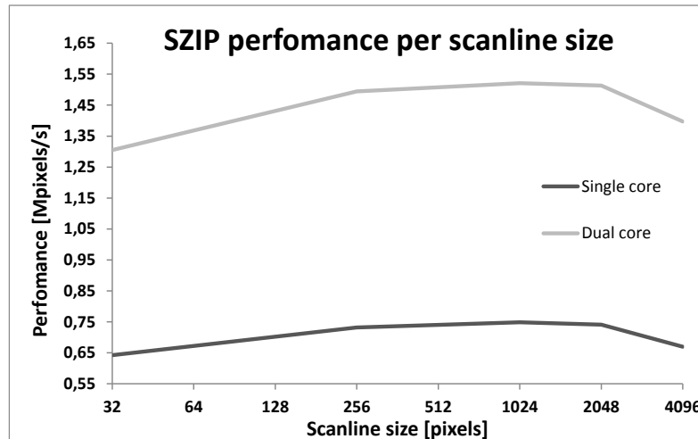
Figure 6: SZIP performance measured in number of compressed Mpxels per second as a function of the scanline size in single and dual core mode
