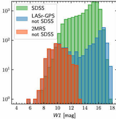
Figure 8. W1 distribution of galaxies within the SDSS spectroscopic core area. Galaxies with SDSS spectra are shown in green, galaxies without but part of the LASr-GPS are shown in blue, and 2MRS galaxies without SDSS spectra in that area are shown in orange.
