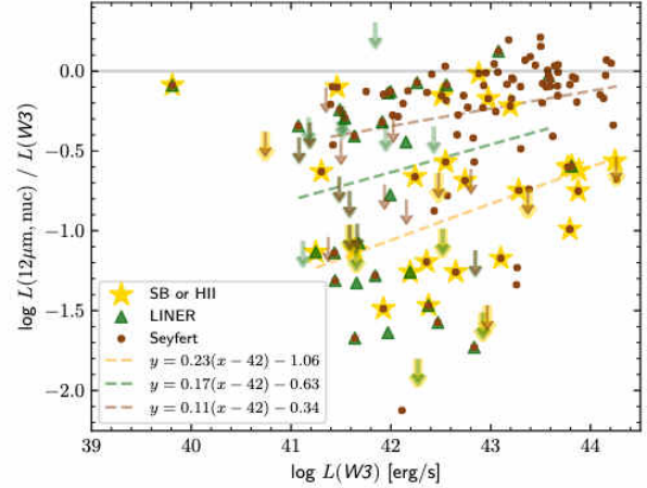
Figure 12. Logarithmic ratio of nuclear 12\mu\text{m} luminosity, L^{\text{nuc}}(12\mu\text{m}) from Asmus et al. (2014) to profile-fitting W3 luminosity, L(W3) , over L(W3) for all 146 objects in common. Objects that are identified as star-forming in the literature (SB or HII) are marked with golden stars, while such with LINER classification have green triangle, and those with Seyfert classifications have brown dots. Objects can have several of these classifications in which cases the corresponding symbols are over-plotted. Nuclear 12\mu\text{m} non-detections are marked by arrows of the corresponding colours. The light grey line marks the zero line, while the dashed lines provide linear fits to various sub-populations of detections, namely the dark grey line for all objects only classified as Seyferts, the green line for Seyferts that also have LINER classification but not star-forming and in orange for all objects without Seyfert classification.
