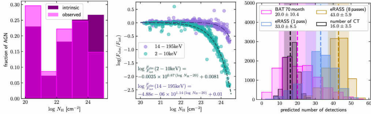
Figure 19. Left: normalised distributions of obscuring column density, N_{\text{H}} , for the BAT 70 month AGN sample. In light magenta is shown the observed distribution for the B70 AGN in LASr fulfilling R90, while in dark purple is shown the inferred intrinsic distribution from Ricci et al. (2015).
