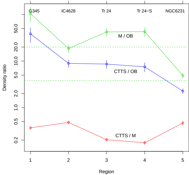
Fig. 19. Net stellar density ratios between M and OB stars, cumulative CTTS and OB stars, and CTTS and M stars, for each subregion. The green dashed lines indicate the maximum and minimum values expected for the M/OB number ratio.
