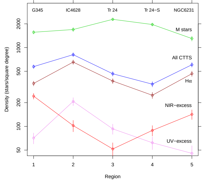
Fig. 18. Spatial density of M stars, H \alpha -excess, NIR-excess, and UV-excess stars for the different regions.
