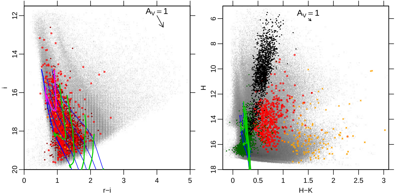
Fig. 9. Color-magnitude diagrams for all stars in the Sco OB1 region ( left panel : (i, r-i) ; right panel : (H, H-K) ). Only data with errors less than 0.1 mag on colors and magnitudes are shown. Colored symbols, tracks, and isochrones as in Fig. 6. The magenta isochrone in the left panel corresponds to 1 M_{\odot} stars. In the (H, H-K) diagram, dark-green dots indicate all candidate M dwarf (or PMS) stars, while black dots are candidate M giants.
