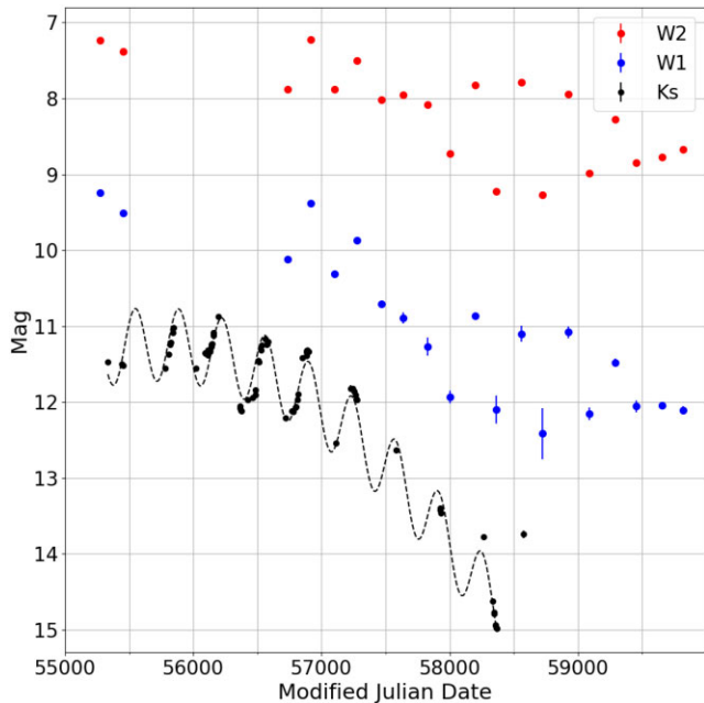
Figure F2. VVV and WISE light curves of source 163. These appear to be a combination of pulsation and a slower, extinction-driven dip. The dashed line shows a simple model fit, see main text. The background grid aids comparison of the amplitude of pulsation in the three filters.
