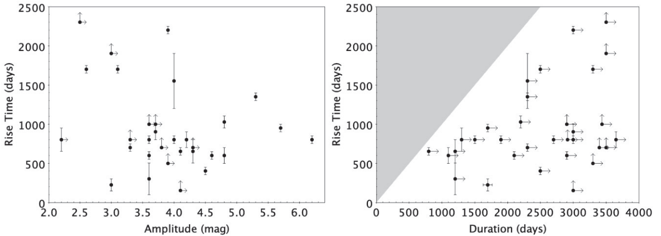
Figure 3. Rise time plotted against amplitude (left-hand panel) and outburst duration (right-hand panel) for 32 classic events drawn from this work and earlier VVV discoveries. Typical rise times are 600–1000 d, though there are faster rises and slower rises. Durations are usually lower limits since the events continued beyond 2019. The shaded region is empty because the duration includes the rise time.
