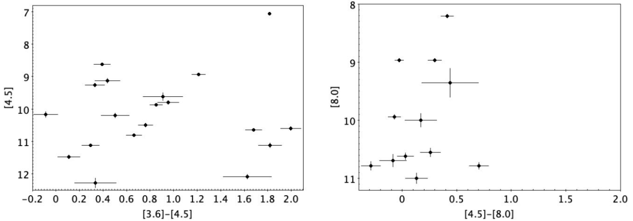
Figure 11. Spitzer /IRAC colour-magnitude diagrams for the dipping giants. ( left-hand panel ): [3.6] - [4.5] versus [4.5] plot for 19 sources. ( right-hand panel ): [4.5] - [8.0] versus [8.0] plot for 12 sources, with the abscissa scaled to emphasize the relatively blue nature of the population in this colour, which is almost independent of extinction. Many sources have [3.6] - [4.5] < 1 , also indicating little emission by hot dust at the time of the GLIMPSE-II survey in 2005–2006, but hot dust is required to explain some sources with [3.6] - [4.5] > 1 .
