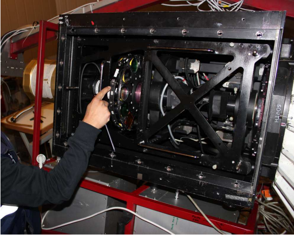
Figure 1. The insides of EFOSC2, mounted on the Nasmyth focus of the NTT. Light enters from the right, the camera is on the left. In between, the two wheels containing filters and gratings can be seen, the finger points at the Wollaston element that was used for the EFOSC2 imaging polarimetry in this paper.
