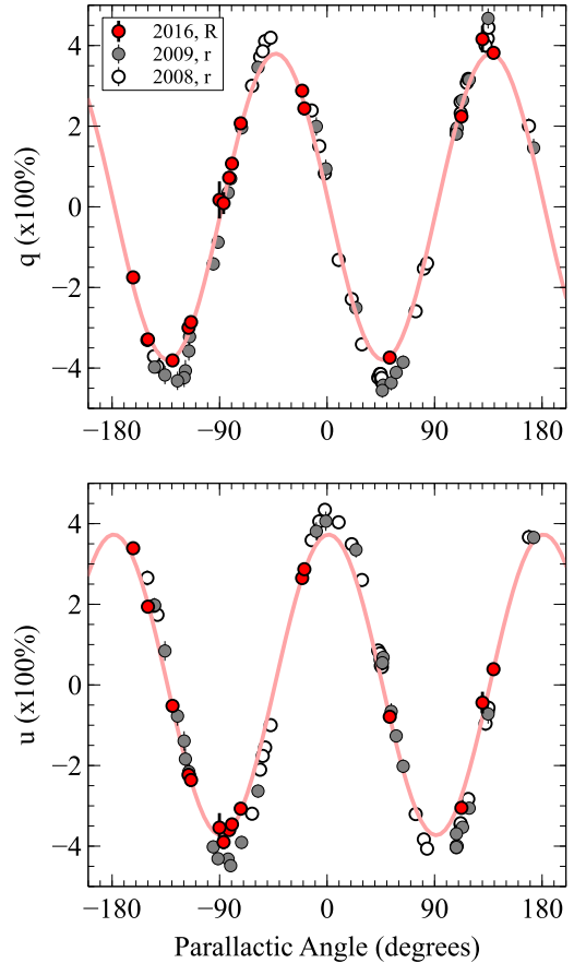
Figure 4. Shown in red are the zero-polarisation standard star datapoints, in instrumental coordinates, from our programme; in grey and white are the data points from Heidt & Nilsson (2011). The thin red line is a cosine fit to our data, to make it easier to see the difference between the data from 2016 and those from 2008 and 2009. A significant change in amplitude can easily be seen, a small phase shift may also be present.
