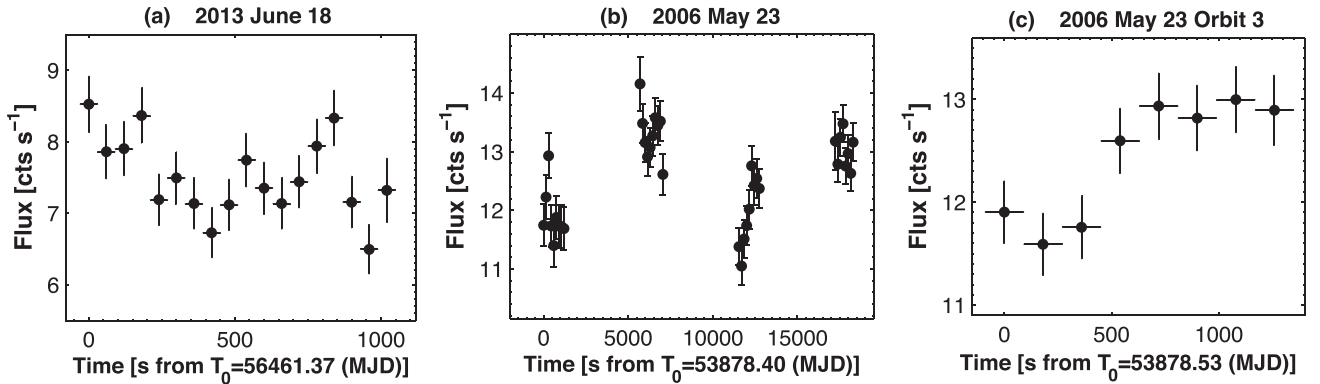
Figure 4. Light curves from the observations with IDVs at the 99.9 per cent confidence (extract).
