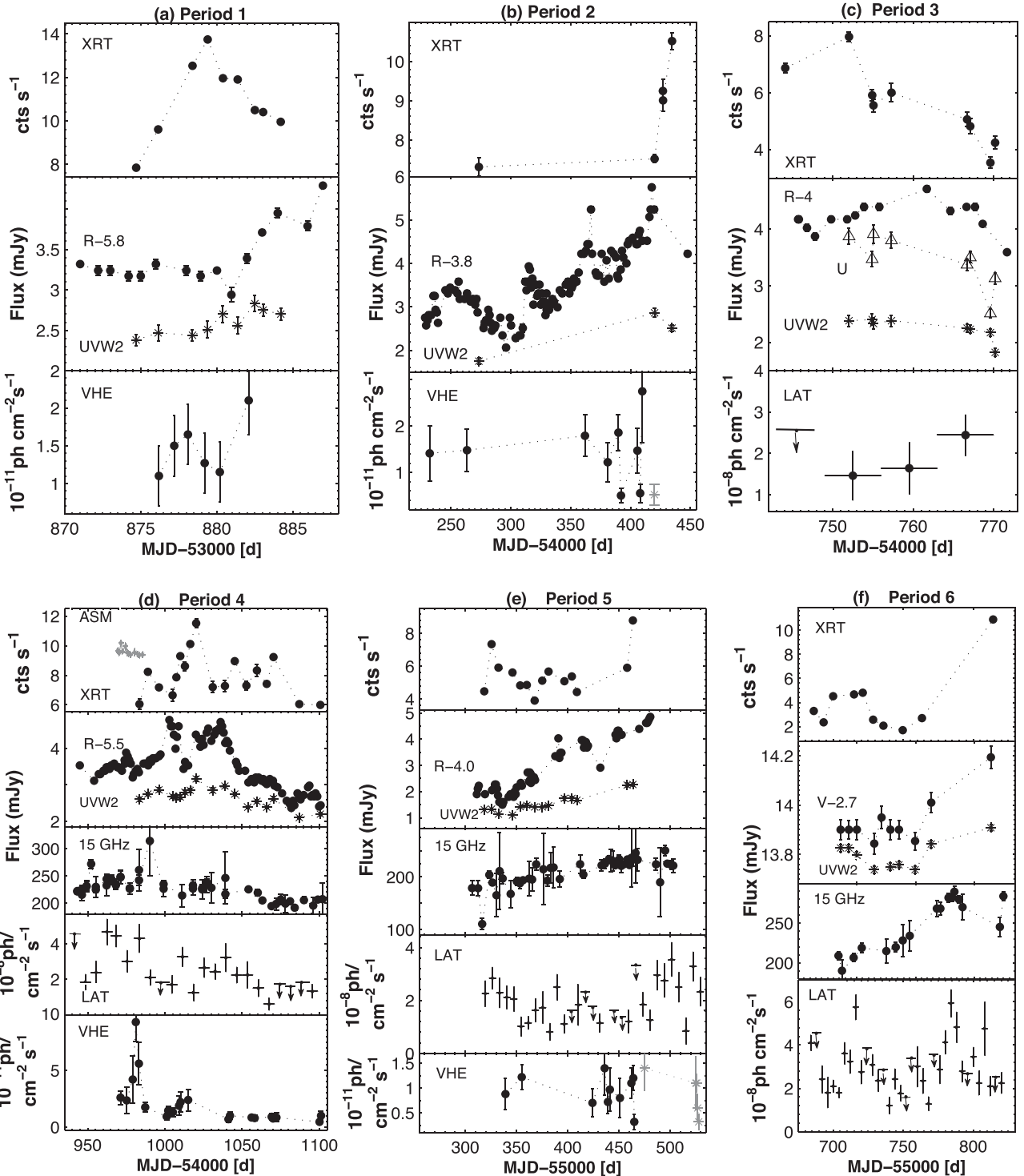
Figure 2. Multi-wavelength variability of 1ES 1959+650 in different epochs.
