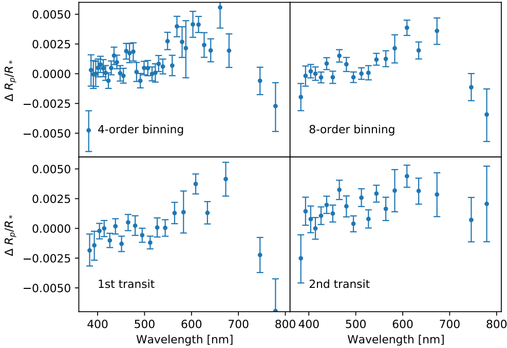
Fig. 4. Transmission spectrum of HD 209458 as obtained from the analysis of the chromatic RM curves. The two upper panels show the combined analysis of the two transits with four- and eight-slice binnings, respectively, for the left and right panels. The two lower panels present the analysis of the two transits separately as computed with an eight-slice binning.
