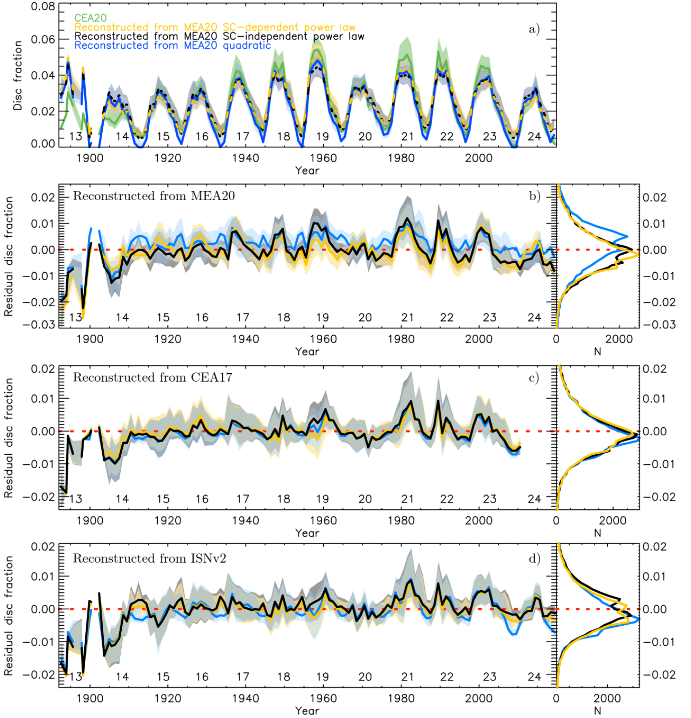
Fig. C.1. Panel a: Reconstructed plage areas from sunspot data along with the CEA20 plage area composite. Shown are annual median values (solid lines) along with the asymmetric 1\sigma intervals (shaded surfaces). The numbers below the curves denote the conventional SC numbering and are placed at SC maximum periods. Panels b–d Left: Residual areas in fractions of the disc between the CEA20 plage area composite and the plage areas reconstructed from the MEA20 sunspot areas (top panels), the CEA17 GSN series (middle panels), and the ISNv2 series (bottom panels). The reconstructions were produced with a simple linear scaling (blue, only for CEA17 GSN and ISNv2), with a squared root function (blue, only for the MEA20 sunspot areas), with a power law function (black), and a power law function with SC-dependent exponents (orange). The red dashed line denotes 0 plage area differences. Panels b–d Right: Distributions of the differences in bins of 0.001 in fractional areas.
