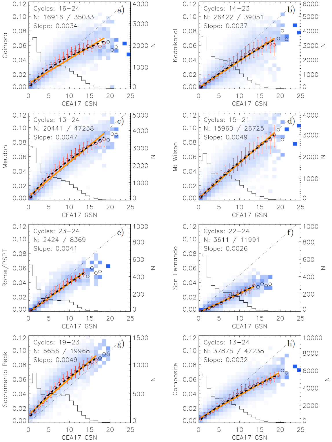
Fig. 3. Same as Fig. 1 but for the CEA17 GSN series. A linear fit (orange) and a power law fit (black dashed) were performed to the mean values of each column. The slope of the linear fit is also listed in each panel. The black dotted line has a slope of 0.005.
