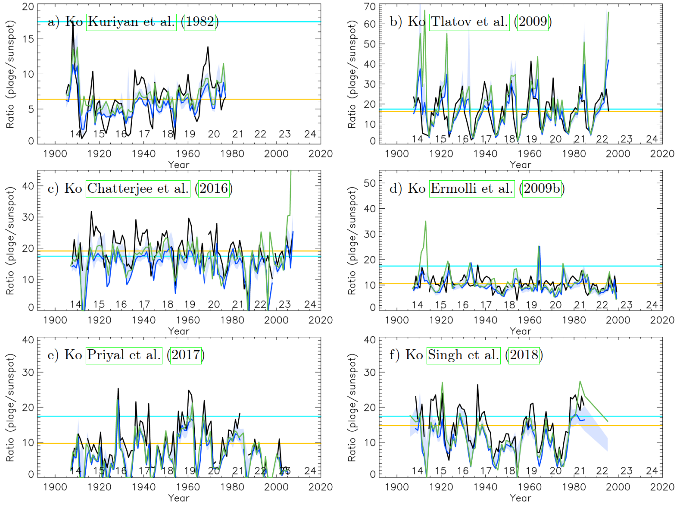
Fig. 6. The ratio of the published plage area series to the sunspot area composite by MEA20 (black), as well as the group sunspot number series by CEA17 (blue) and SvSc16 (green). The plage area series shown are those for Ko data by Kuriyan et al. (1982, a)), Tlatov et al. (2009, b)), Chatterjee et al. (2016, c)), Ermolli et al. (2009b, d)), Priyal et al. (2017, e)), and Singh et al. (2018, f)). The first two series provide only annual mean values, while the others have daily cadence. The ratios to the group sunspot number series have been multiplied by 2000 to be plotted alongside the ratios to the sunspot areas. The blue shaded surface denotes the range of annual values for the ratios from all the sunspot number series used in this study (see Sect. 2). The solid lines are annual median values. The ratios for the series with daily values are calculated only for the days for which the plage areas are greater than 0.0005 in disc fraction. The yellow (light blue) horizontal line represents the average ratio value between the MEA20 sunspot areas and the corresponding plage series (the CEA20 composite plage area series). The numbers at the lower part of each panel denote the conventional SC numbering and are placed at SC maximum periods.
