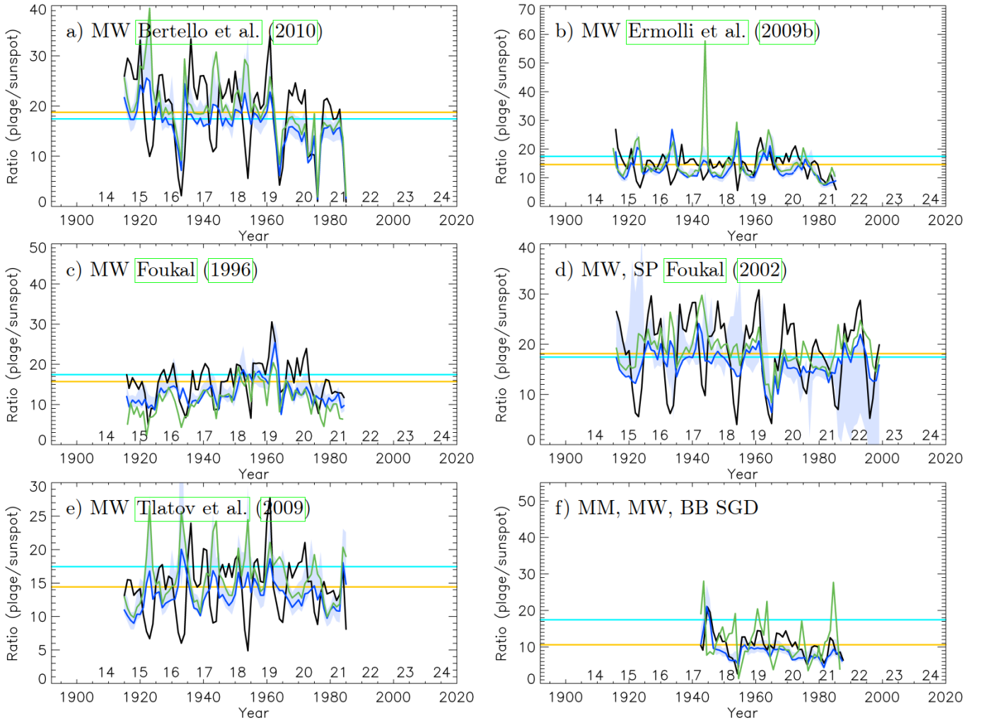
Fig. 7. Same as Fig. 6 but for the plage area series for MW data by Bertello et al. (2010, a); MW data by Ermolli et al. (2009b, b); MW data by Foukal (1996, c); MW and SP data by Foukal (2002, d); MW data by Tlatov et al. (2009, e); and for MM, MW, and BB data by SGD (f). The series in panels b), c) and f) have daily values, while the others have only annual mean values. The Bertello et al. (2010) series, which is a Ca II K emission index series, was linearly scaled to match the plage areas from our MW data (see Sect. 2).
