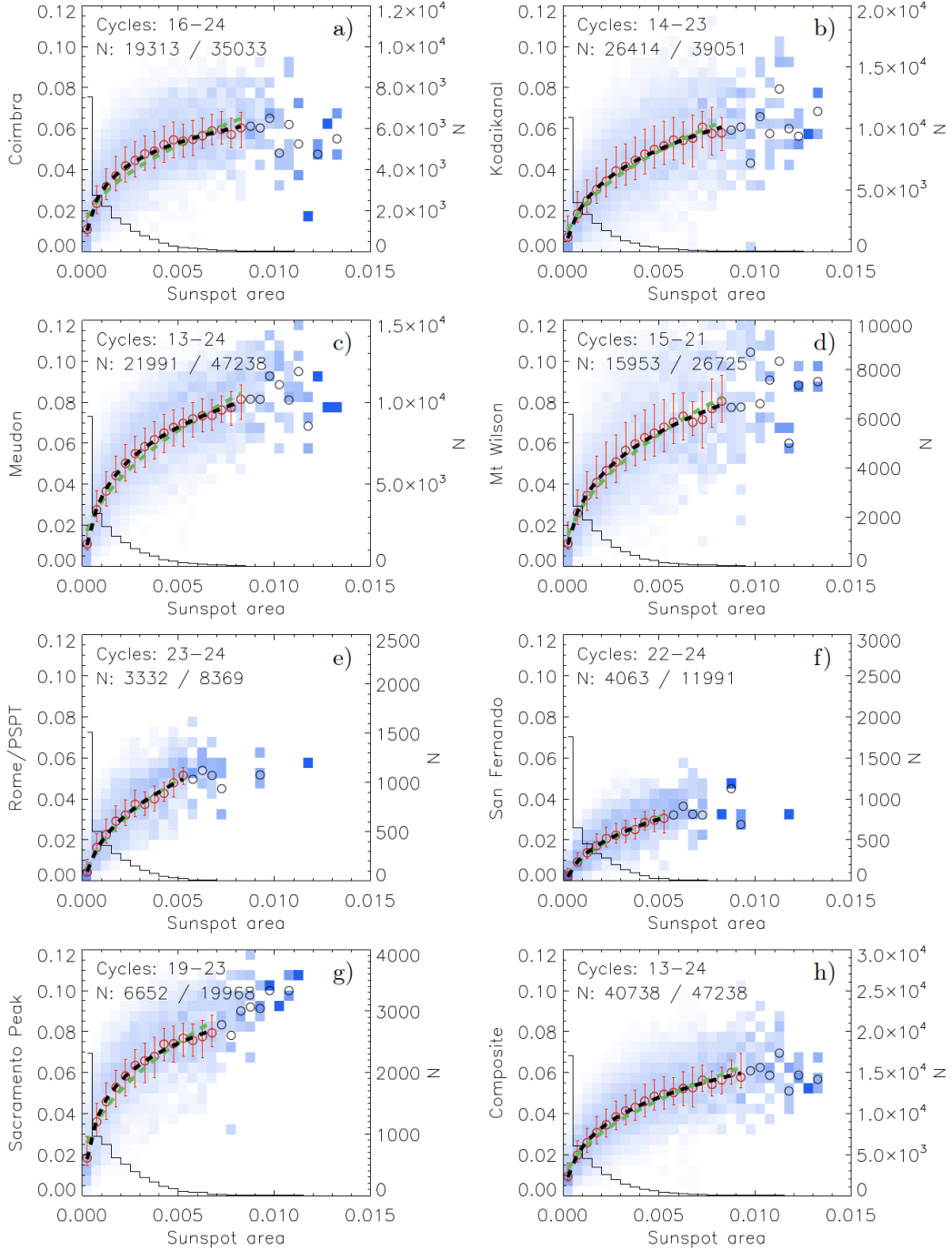
Fig. 1. Probability distribution functions (PDF) for plage fractional areas as a function of the sunspot fractional areas from MEA20. Both plage and spot areas were taken on the same days. The PDFs are shown in bins of 0.005 and 0.0005 fractional areas for plage and sunspots, respectively. Each panel shows the PDF matrix for a given Ca II K archive; Co (a)), Ko (b)), MD (c)), MW (d)), RP (e)), SF2 (f)), SP (g)), and the CEA20 plage area composite (h)). The PDFs are colour-coded between white for 0 and bright blue for 1. Circles denote the average plage area value within each column. For columns with less than 20 days of data these circles are shown in black, otherwise in red. We also show the asymmetric 1\sigma interval for each column. Two different fits to the average values are over-plotted, a power law fit (black), and a square root function (green). The number of days included in each column is also shown as a solid black histogram (see right-hand axis). The period of overlap between the two archives shown in a given panel (expressed in solar cycles), as well as the total number of overlapping days used to construct each matrix (N) and the total number of days within this time interval are listed in the top part of each panel.
