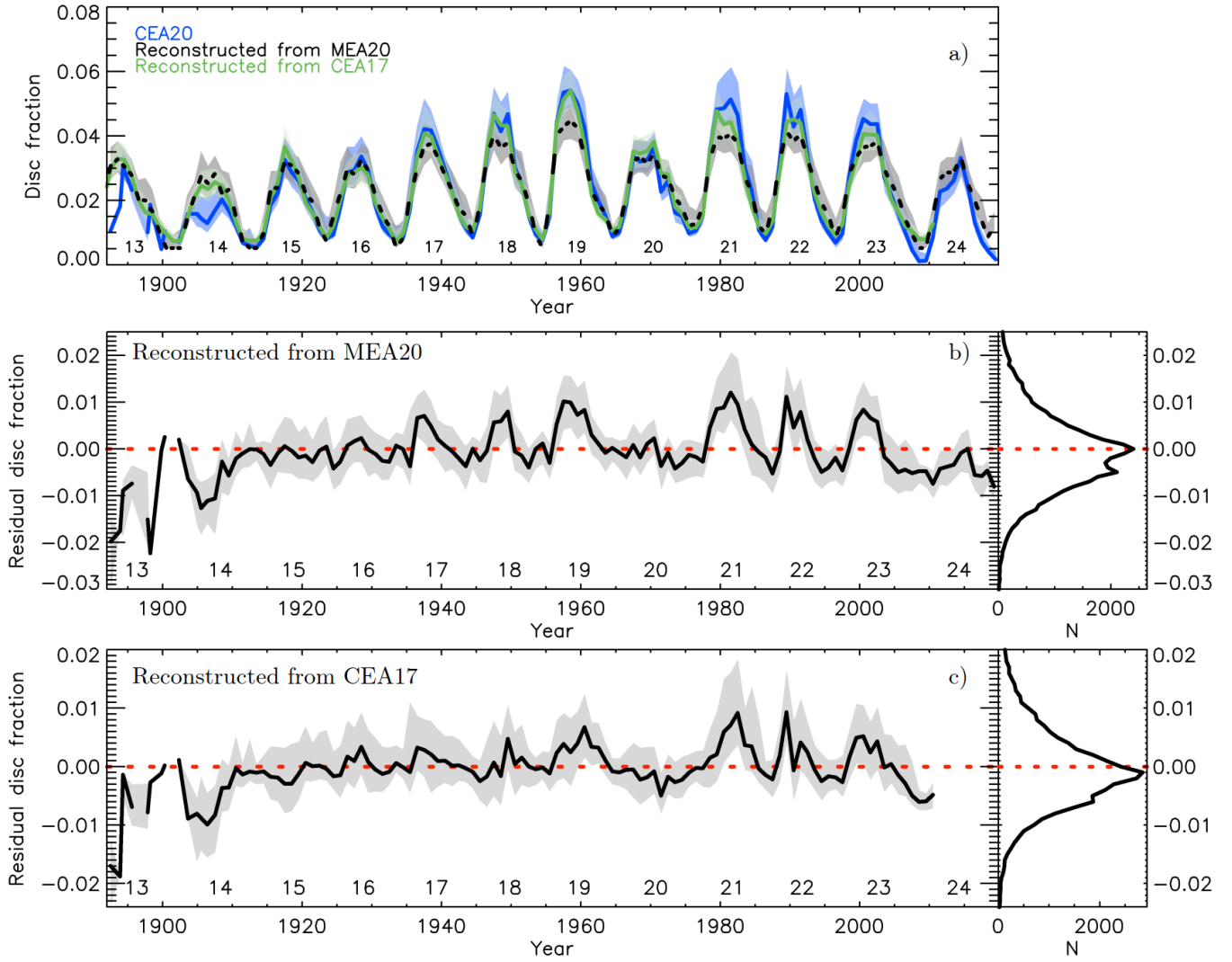
Fig. 5. Panel a: Reconstructed plage areas from MEA20 sunspot area series (black) and the CEA17 GSN series (green) along with the CEA20 plage area composite (blue). Shown are annual median values (solid lines) along with the asymmetric 1\sigma intervals (shaded surfaces) only for the period covered by CEA20 plage area composite. The numbers below the curves denote the conventional SC numbering and are placed at SC maximum periods. Panels b–c Left: Residual areas in fractions of the disc between the CEA20 plage area composite and the plage areas reconstructed from the MEA20 sunspot areas (panel b) and the CEA17 GSN series (panel c). The red dashed line denotes 0 plage area differences. Panels b–c Right: Distributions of the differences in bins of 0.001 in fractional areas.
