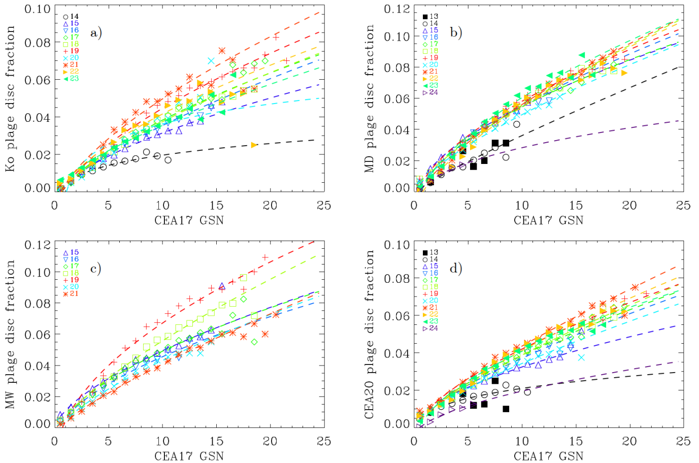
Fig. A.2. Relation between plage areas and CEA17 GSN for individual SC based on the data from the Ko (a), MD (b), and MW (c) archives as well as the CEA20 plage area composite (d). Shown are the binned values along with power law fits. The lines are coloured according to the strength of the SC with the strength increasing from black for the weakest cycle, via dark blue, turquoise, green, lime, orange, bright red to dark red for the strongest SC.
