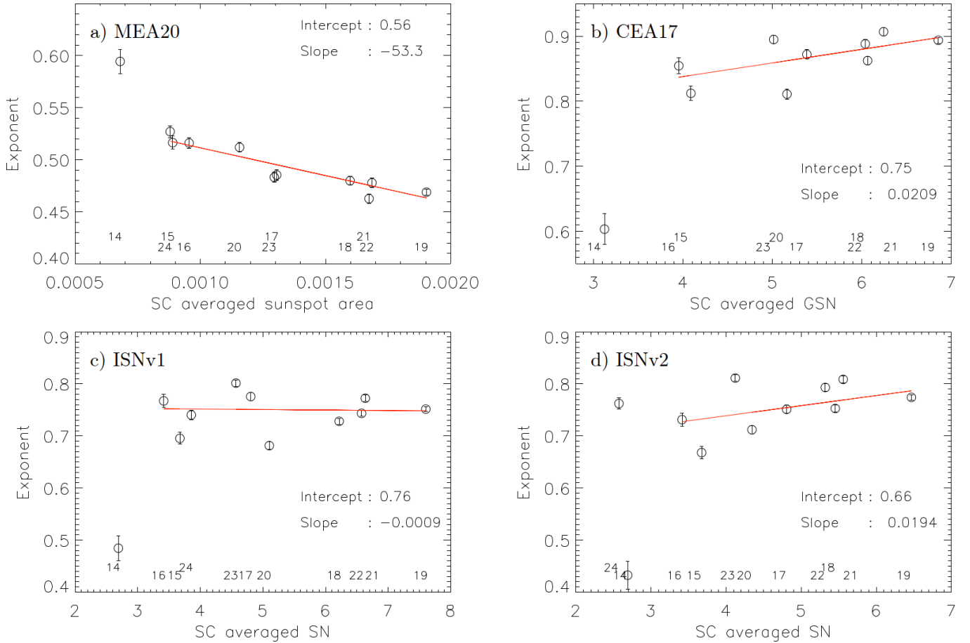
Fig. A.4. Exponents of power law fits to the relation between the CEA20 plage area composite and MEA20 (panel a) sunspot areas as well as CEA17 GSN (panel b), ISNv1 (panel c), and ISNv2 (panel d) series plotted as a function of SC average sunspot number. Solid red lines are linear fits to the individual SC values excluding SCs 13 and 14, which do not have enough statistics in the plage area composite. For the comparison to the sunspot number series we also excluded SC 24 since the CEA17 GSN series ends in 2010, while ISNv1 in 2014. The parameters of the linear fits are also given in each panel. Numbers within the panels denote the conventional SC numbering.
