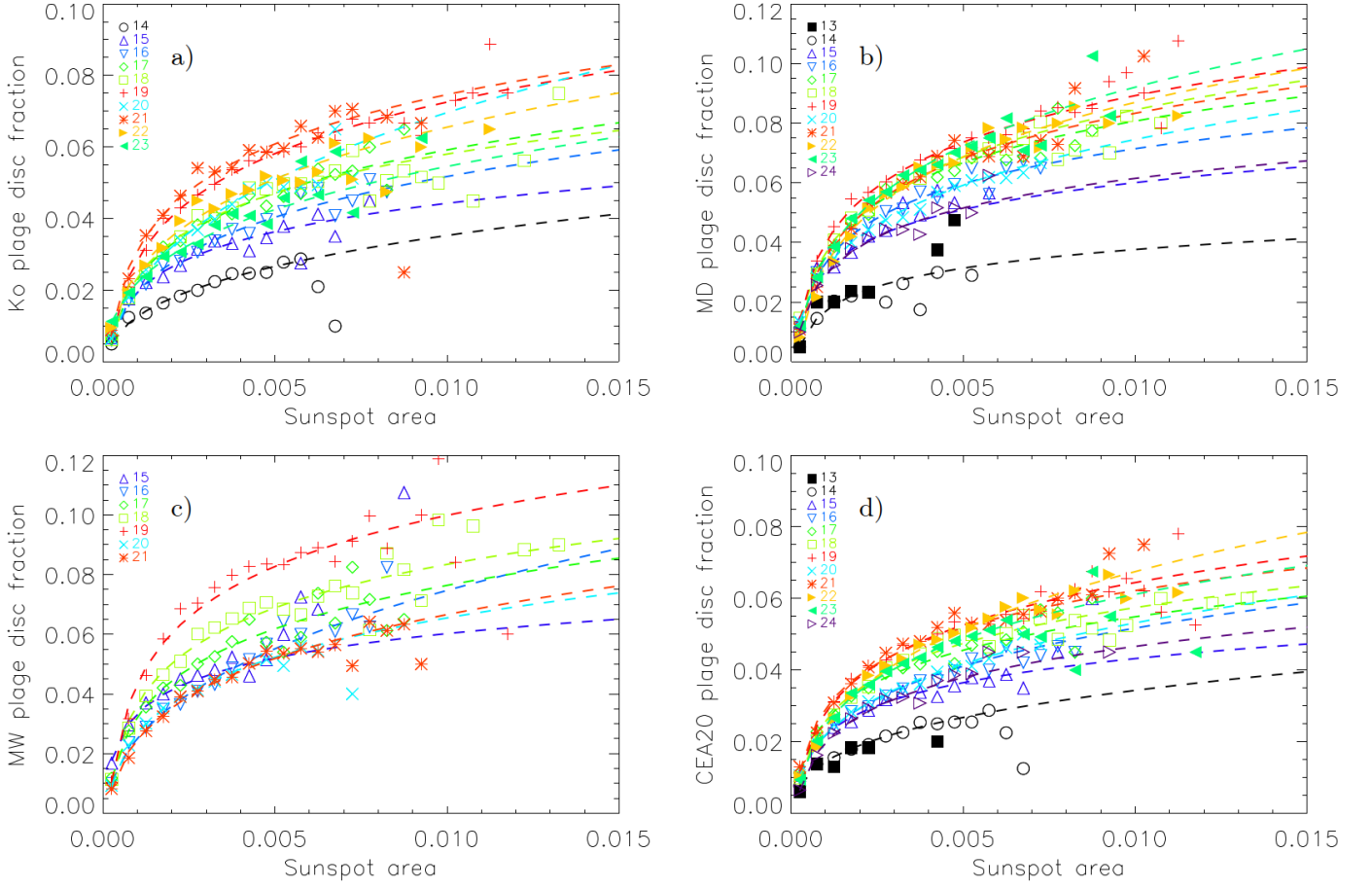
Fig. A.1. Relation between plage and sunspot areas for individual SC based on the data from the Ko (a), MD (b), MW (c) archives, and the CEA20 plage area composite (d). The symbols denote the mean values of the PDF matrices (as shown in Fig. 3). The dashed lines are power law fits and are coloured according to the strength of the SC with the strength increasing from black for the weakest cycle, via dark blue, turquoise, green, lime, orange, bright red to dark red for the strongest SC.
