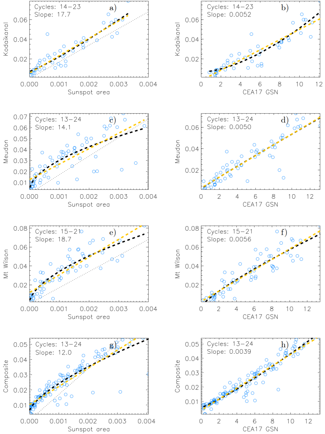
Fig. 2. Scatter plots between annual plate fractional areas and the annual MEA20 sunspot fractional areas (left columns) as well as the annual CEA17 GSN series (right columns). Two different fits are over-plotted, a power law (black) and a linear (yellow) fit. The dotted line has a slope of 17, which corresponds to the mean ratio between the CEA20 plate area series and the MEA19 sunspot area series (see Sect. 3.1). The period of overlap between the two archives (expressed in solar cycles) as well as the slope of the linear fit are shown in each panel.
