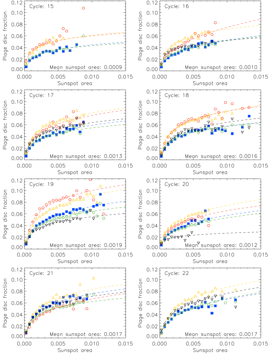
Fig. A.3. Similar to Fig. A.1, but now each panel shows the relationships for Co (black downward triangles), Ko (blue squares), MD (orange upward triangles), MW (red circles), and CEA20 composite (green circles) series for individual SCs 15 to 22, as specified in each panel. Also listed in each panel is the cycle-averaged sunspot fractional area.
