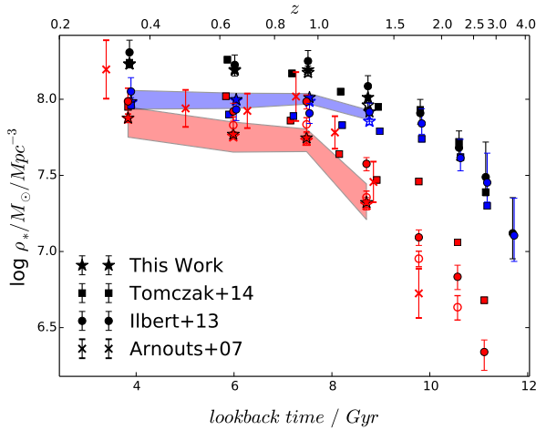
Fig. 16. Evolution of the cosmic stellar mass density for all (black), star-forming (blue), and quiescent (red) galaxies. The shaded areas show the corresponding systematic uncertainties that are due to the SF/Q selection. The open stars represent the measurement that we obtain by assuming a single-Schechter function to fit the star-forming galaxies. Measurements of Tomczak et al. (2014, squares), Ilbert et al. (2013, circles), and Arnouts et al. (2007, quiescent only, red crosses) are shown for comparison. The filled and open red circles represent the quiescent measurements of Ilbert et al. (2013), using a selection of quiescent galaxies based on the NUV-r/r-J plan and the sSFR respectively. The quiescent measurement of Arnouts et al. (2007) is based on the K -band luminosity density, and the selection uses the SED-fitting. For the sake of clarity, the star-forming or quiescent measurements are plotted with a shift of +0.03 or -0.03 Gyr.
