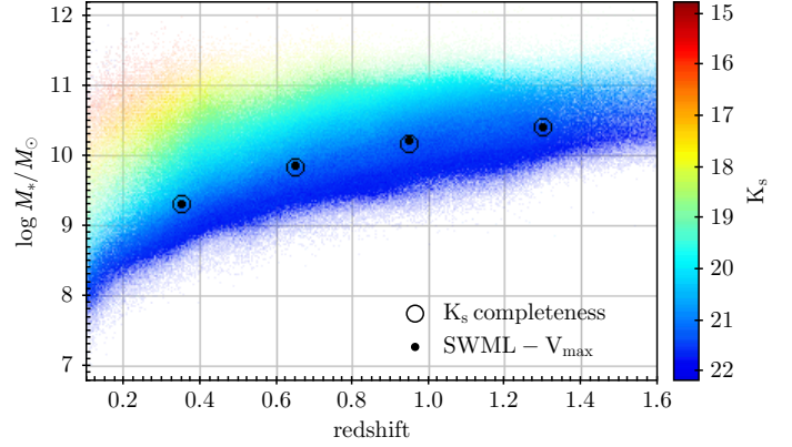
Fig. 4. Stellar mass versus redshift for our K_s < 22 -limited sample of galaxies. The black open circles represent the stellar mass completeness limit computed with the K_s completeness limit M_{\text{lim}} according to Eq. (1). The black dots represent the mass at which the V_{\text{max}} and the SWML SMF estimators diverge (see below Sect. 5.1).
