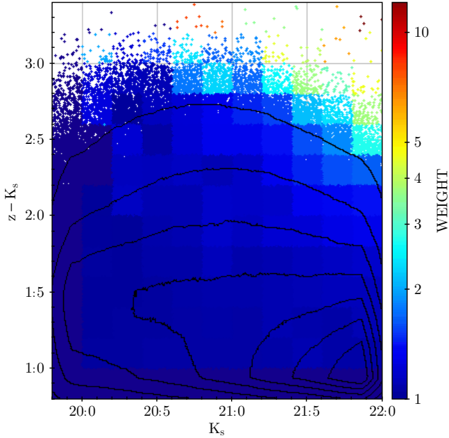
Fig. 2. Colour–magnitude weight map used for our statistical analysis. It takes the missing objects in the K_s < 22 -limited sample into account. These objects are missed because the gri -detection was used to extract the K_s fluxes. Weights are multiplicative. This map is restricted to galaxies with redshift z \leq 1.5 (cf. Sect. 3) and the contours outline the galaxy density distribution.
