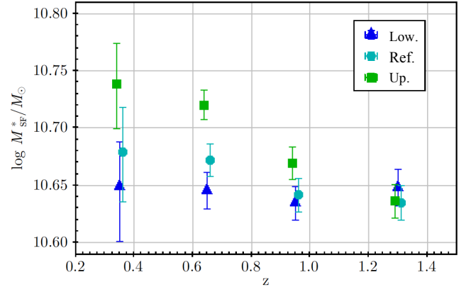
Fig. 17. Redshift evolution of M_{SF}^* , corresponding to the three selections of SF galaxies in the NUVrK diagram defined in Sect. 5.1: the reference selection (for which the limit lies in the middle of the green valley; cyan circles), its lower limit (when galaxies in transition are excluded; blue triangles), and the upper limit (if the green valley is included in the SF locus; green squares).
