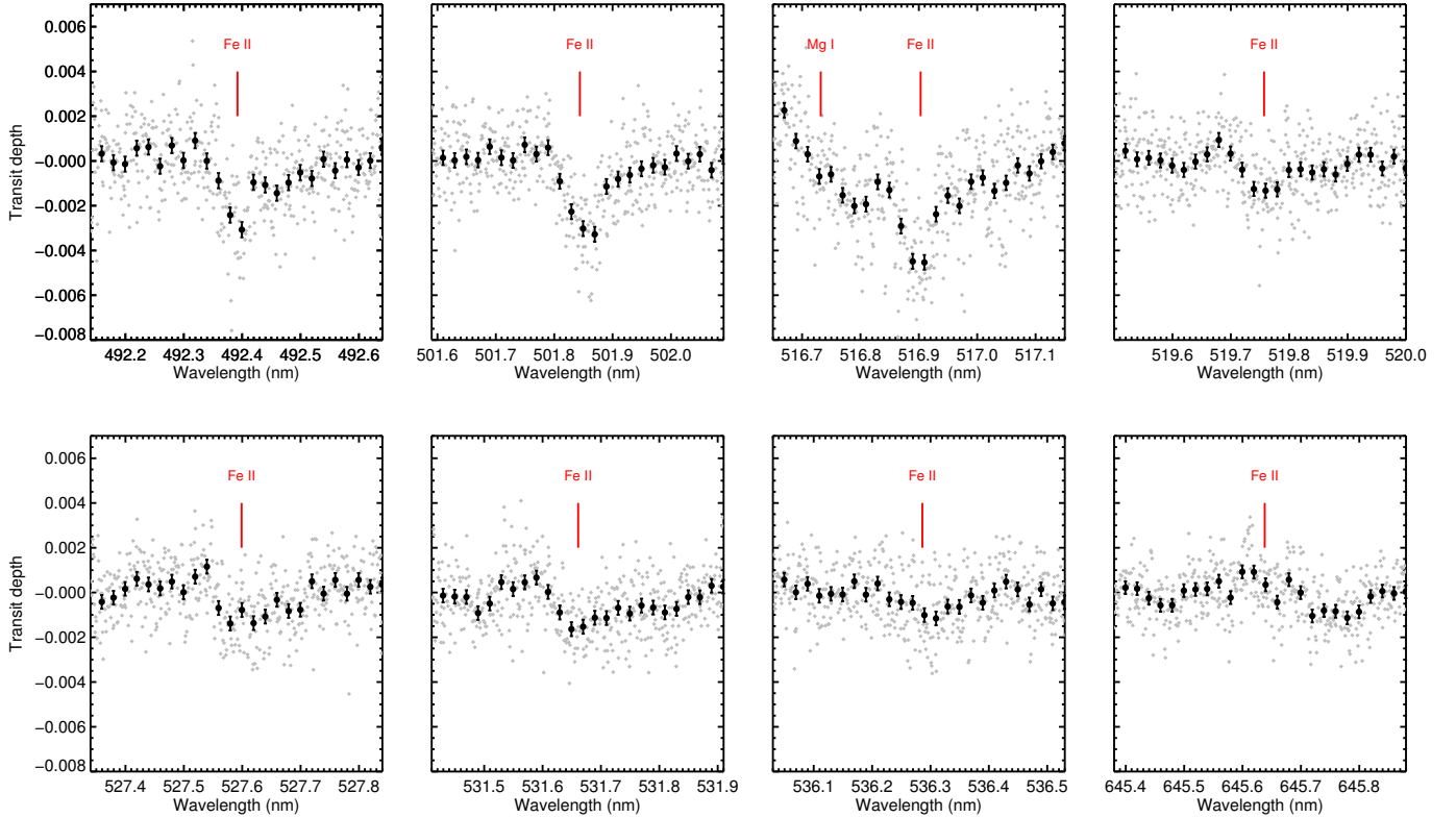
Fig. 7. Transmission spectrum of KELT-9 b at the location of eight strong lines of Fe II that were observed by Cauley et al. (2019) . The grey points show the transmission spectrum at the native sampling of the HARPS-N instrument, while the black points are binned by 20 points. The transmission spectrum is obtained following the procedure of Wytenbach et al. (2015) , and combining all in-transit exposures of the two nights. The Doppler-shadow is removed by fitting the model described in Sect. 2 at the expected locations of the individual lines. The presence of these lines appears to be confirmed by our HARPS-N observations, but non-Gaussian systematic noise occurs at the \sim 10^{-3} level. This hinders the identification of all but the strongest Fe II lines.
