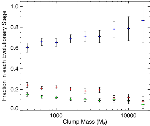
Figure 26. Fractions of clumps sorted by evolutionary stage. The green, red and blue circles indicate the fractions of quiescent, protostellar and mid-IR bright clumps (YSOs and MSF clumps), respectively, as a function of clump mass. The uncertainties are determined from Poisson counting statistics. This plot only includes mass bins above the nominal survey completeness ( \sim 400 M_{\odot} ), and averages the source counts in bins of 0.2 dex.
