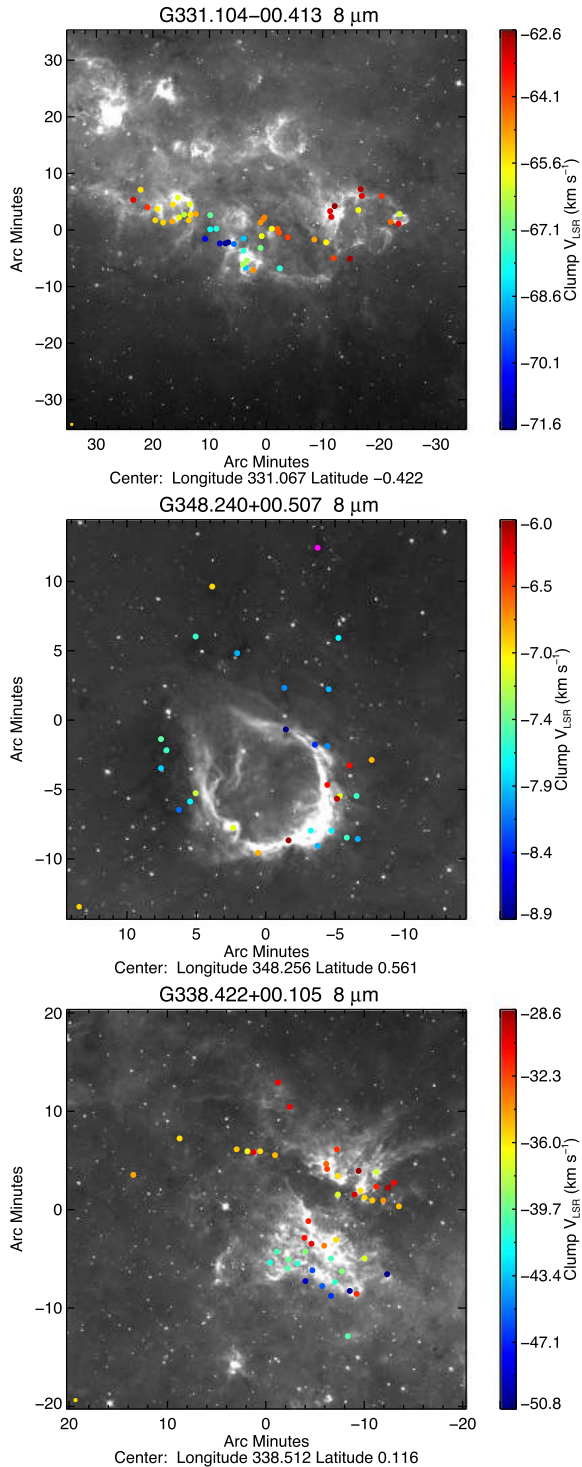
Figure 30. ATLASGAL clusters associated with MPC candidates identified by Contreras et al. (2017) and Longmore et al. (2017) identified by the friends-of-friends analysis. The background image is the 8 μm emission and filled circles show the positions of ATLASGAL CSC objects, the colours of which provide an indication of their velocities (see colour bars for values).
