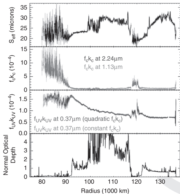
Figure 3.25 Bottom: Standard \tau profile; first panel up: f_{UV}k_{UV} for the UV-absorbing material as mapped by the 0.35–0.55 \mu\text{m} slope (with negligible dependence on the assumed form of the “constant” absorber); second panel up: f_c k_c for the weakly reddish, possibly silicate, material as mapped by the 0.55–0.90 \mu\text{m} slope; top panel: “effective” grain diameter S_{eff} consistent with the above determinations and the observed water ice band depths. Adapted from Hedman et al. (2013a).
