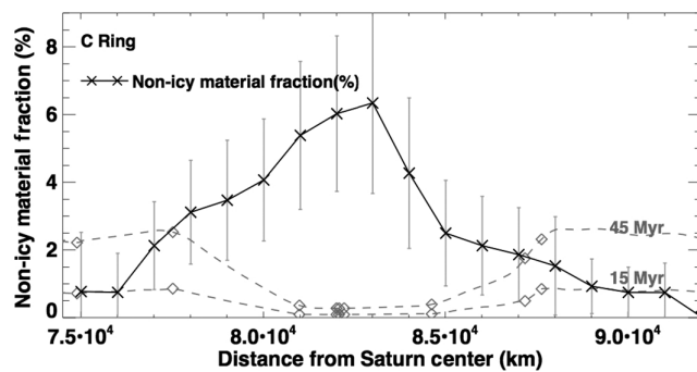
Figure 3.19 Black curve: Non-icy material fraction derived from Cassini 2 cm radiometer observations. Grey dashed curve: The non-icy material fraction as evolved over 15 and 45 Myr if meteoroid bombardment is the only source of contamination in a structurally fixed ring, and the flux has remained constant. Grey diamonds indicate locations where opacity measurements have been made through density waves. Figure adapted from Zhang et al. (2017).
