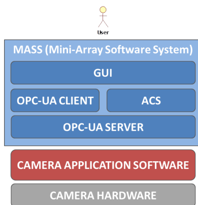
Figure 5. Software layers of the ASTRI SST-2M Camera
