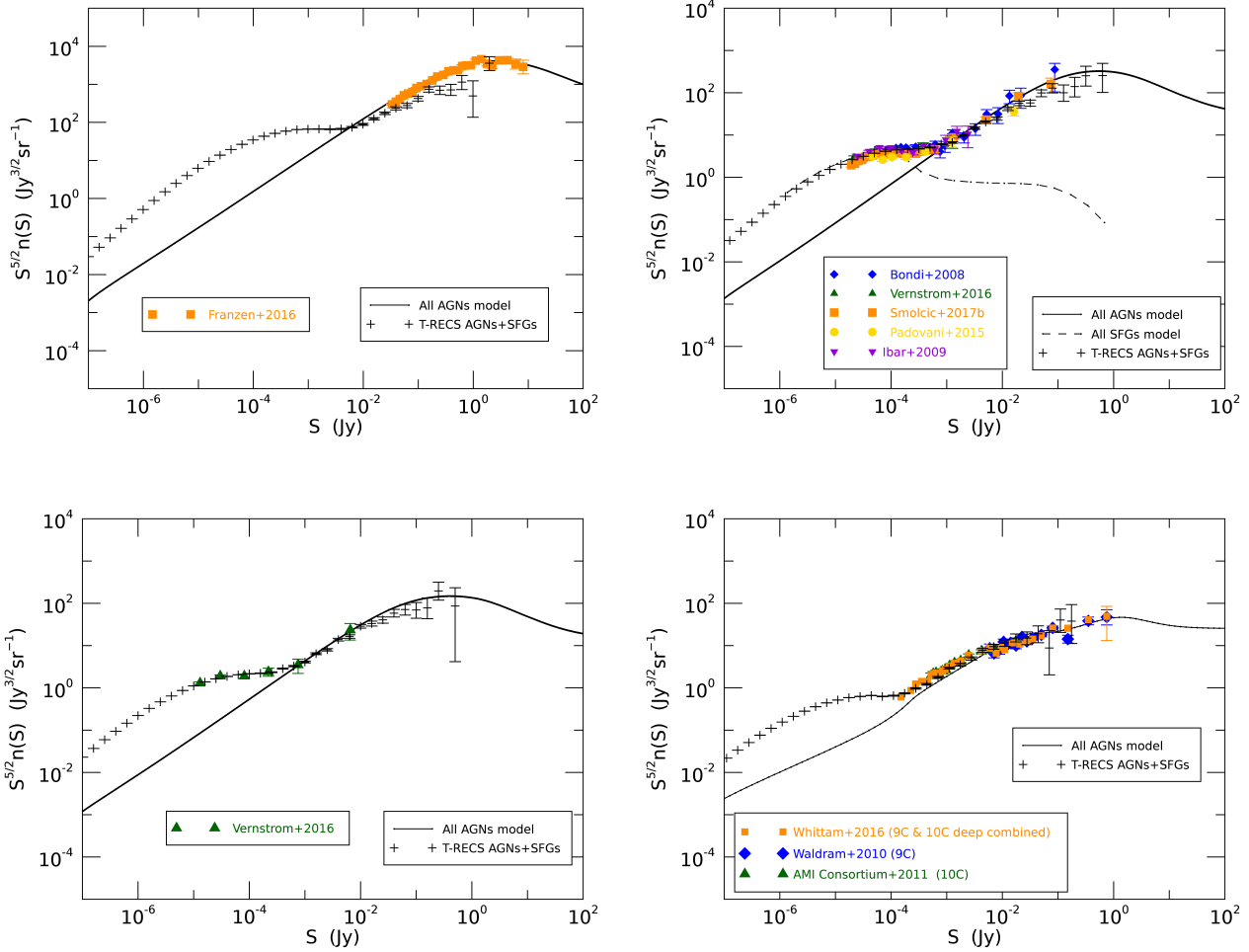
Figure 6. Comparison of differential source counts in total intensity at 150 MHz (top left) 1.4 GHz (top right), 3 GHz (bottom left) and 15 GHz (bottom right) between T-RECS, models from Bonato et al. (2017) and the available data from Franzen et al. (2016); Bondi et al. (2008); Vernstrom et al. (2016); Smolčić et al. (2017b); Padovani et al. (2015); Ibar et al. (2009); Whittam et al. (2016); Waldram et al. (2010); AMI Consortium et al. (2011).
