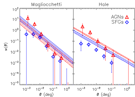
Figure 10. Two-point angular correlation function w(\theta) yielded by our simulation for radio AGNs and SFGs (points with error bars) compared to the results of Magliocchetti et al. 2017 (left) and Hale et al. 2018 (right) for the same populations (shaded areas represent the best fit \pm 1 \sigma uncertainty in the normalization).
