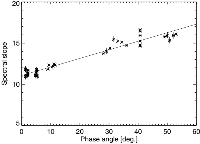
Fig. 3. Variation of the mean spectral slope of the nucleus of 67P, evaluated in the 882–535 nm range and expressed in \%/(100 \text{ nm}) , with the phase angle.
