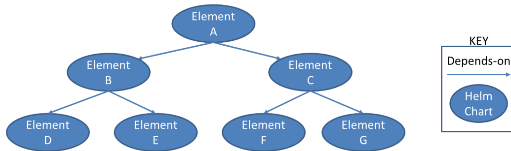
Figure 4. SKAMPI
