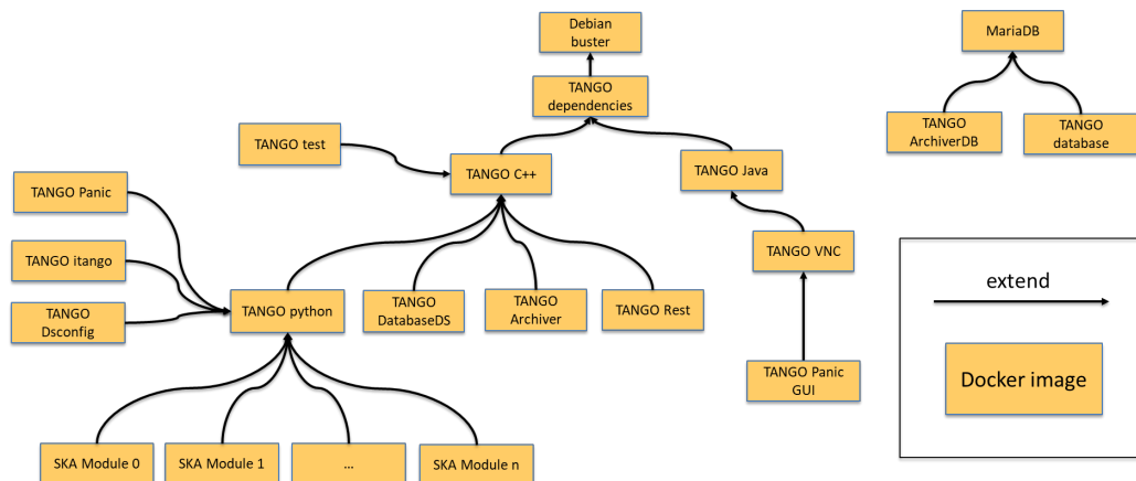
Figure 2. SKA-Docker repository
