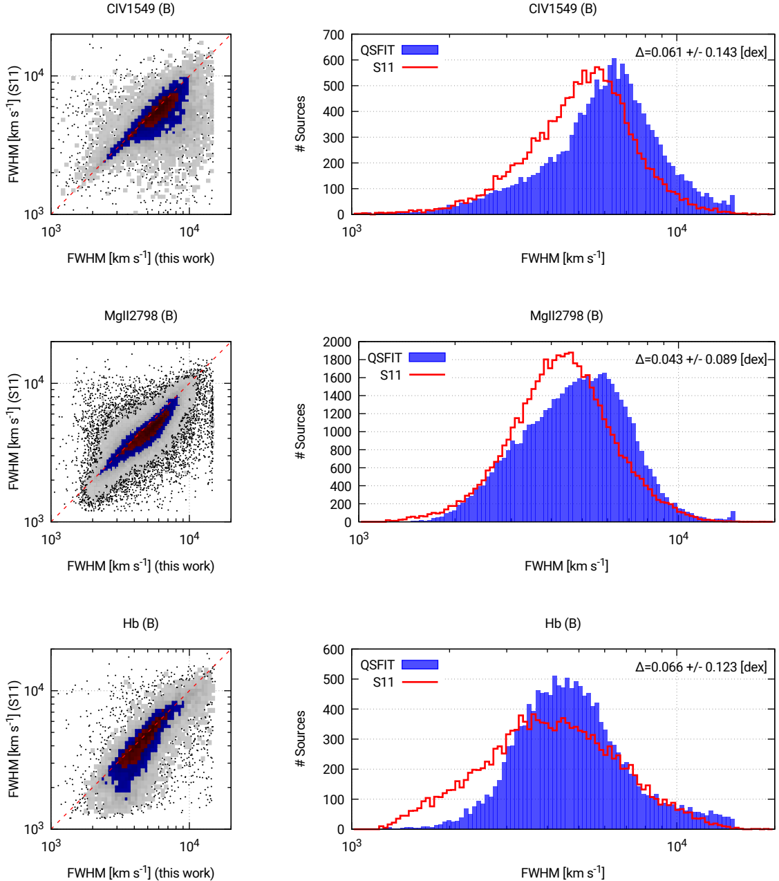
Figure 14. Comparison of QSFIT and S11 broad component widths of CIV 1549Å, MgII 2798Å and Hβ 4861Å emission lines. The plot meaning is the same as in Fig. 10. The discrepancies are mainly due to the different line profile decomposition.
