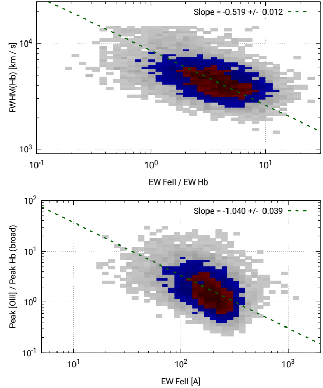
Figure 16. Correlations between the width of the broad Hβ emission line (upper panel) and the peak luminosity ratios between [O III] and Hβ (lower panel) vs. the [Fe II] equivalent width, using the data from the QSFIT catalog.
