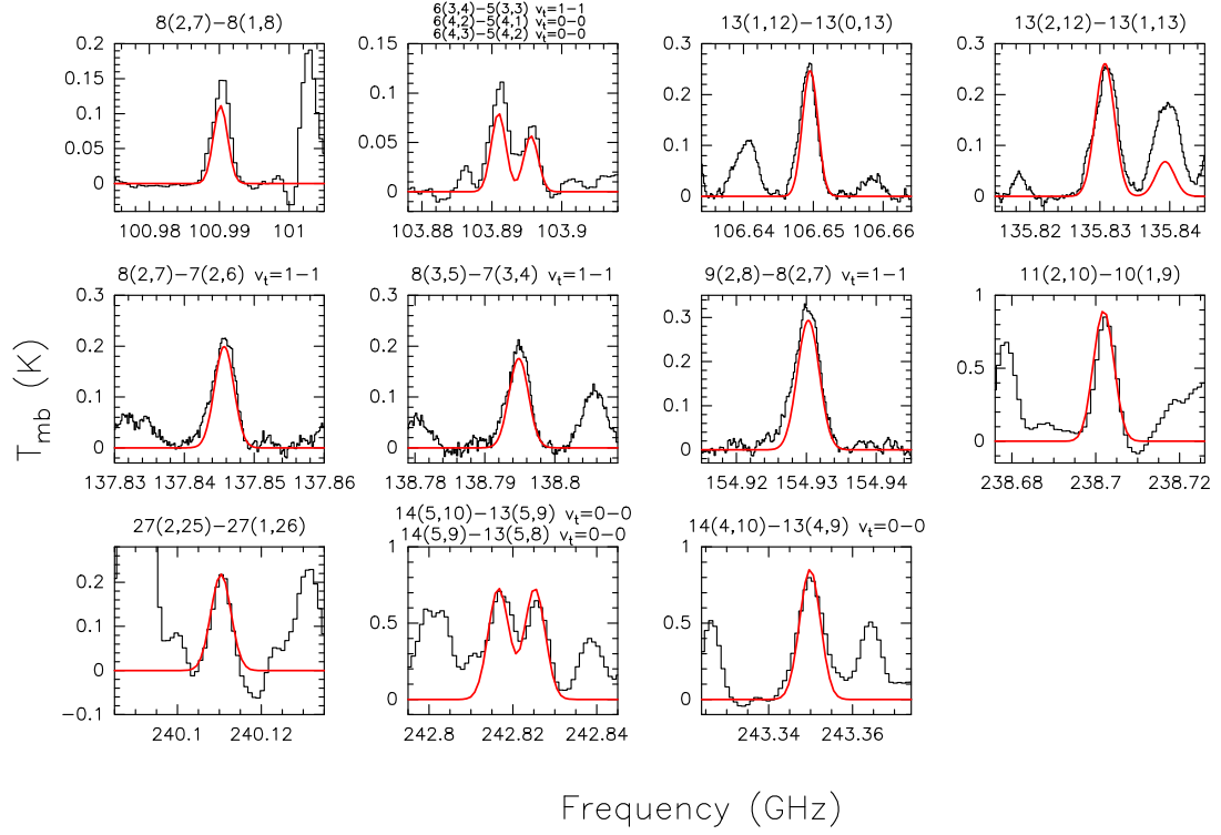
Fig. A.2. Selected unblended transitions of ET (see Table A.2) with LTE fit (red line).
