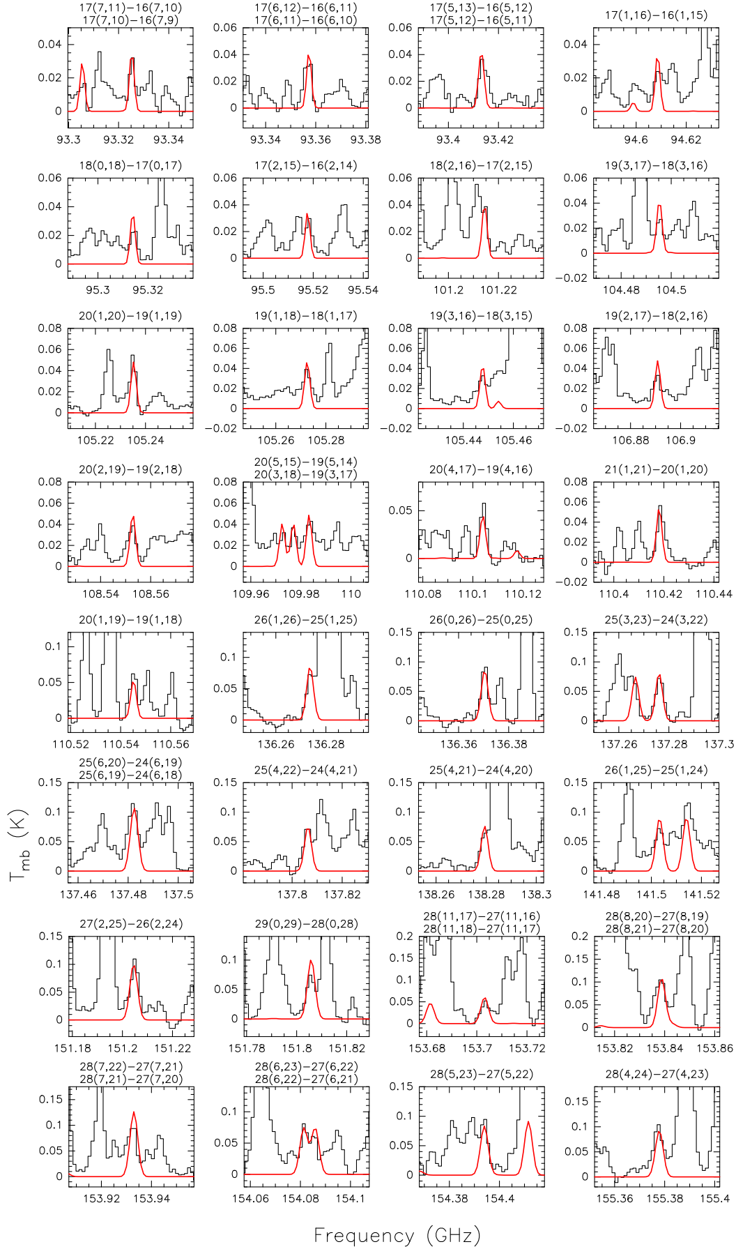
Fig. 1. Unblended or slightly blended transitions of the trans conformer of EF towards the W51 e2 hot core (see Table 2). We have overplotted in red the LTE synthetic spectrum obtained with MADCUBAIJ assuming a temperature of 78 K, a column density of 2 \times 10^{16} \text{ cm}^{-2} and a source size of 2.4'' .
