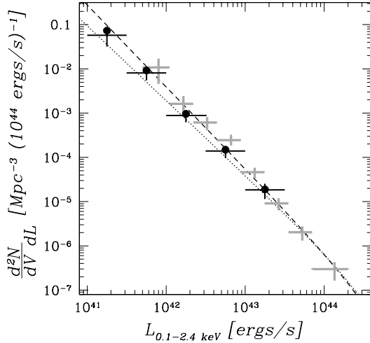
Fig. 16. X-ray luminosity function of ECDF-S groups. Black dots show the measurement using the full field, while black crosses show the measurements excluding the central region where there is a low spatial density of groups. Gray crosses show the results from the COSMOS field. Dashed and dotted curves show the local XLF in the Northern and Southern Hemisphere, revealing an effect of sample variance, caused by small volumes probed by RASS at low group luminosities.
