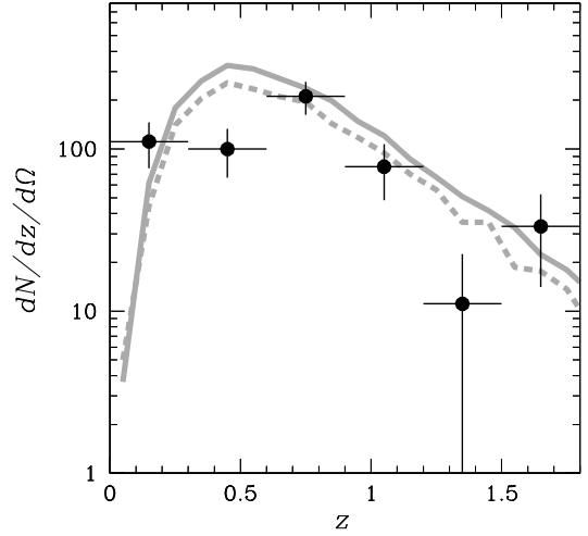
Fig. 18. dn/dz/d\Omega [deg ^{-2} ] distribution of the ECDF-S groups (black crosses). The prediction from the detailed detection simulation and Planck cosmology (Planck Collaboration XXVI 2014) is shown as solid grey curve and the effect of 30% change in the scaling relations is shown by the dashed grey curve.
