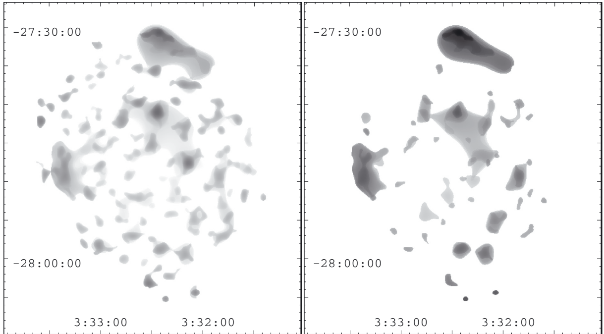
Fig. 3. Wavelet reconstruction of the XMM image on 32''–128'' scales without ( left panel ) and with ( right panel ) the flux removal coming from the wings of point sources. The number of apparent sources changes by a factor of 2.
