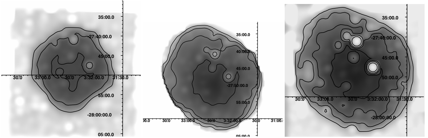
Fig. 2. Sensitivity of Chandra and XMM towards the detection of X-ray emission on 32'' scales. Contours show the levels of 1.2, 2, 3, and 5 \times 10^{-16} ergs s ^{-1} cm ^{-2} and provide the intensity scale in the image. Left: all Chandra observations. The sensitivity does not reach the deepest contour. Middle: All XMM observations. Right: Chandra plus XMM.
