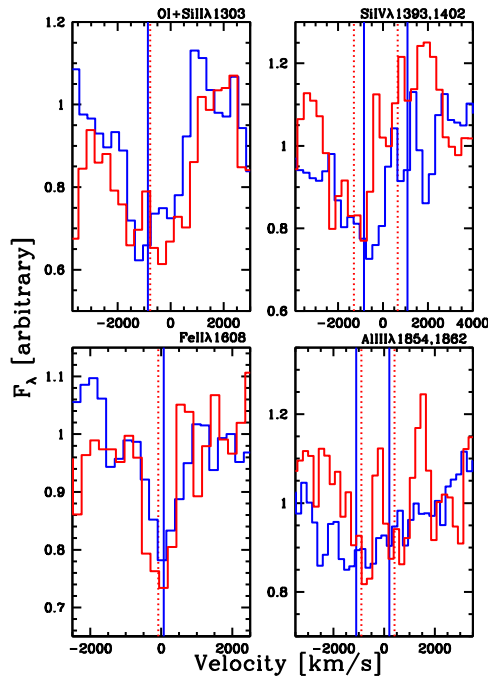
Figure 9. ISM absorption lines in the stacked spectra of individually detected X-ray AGN with L_X > 10^{43.6} \text{ erg s}^{-1} (red); individually detected X-ray AGN with L_X < 10^{43.6} \text{ erg s}^{-1} (blue), relative to zero velocity defined by the He II \lambda 1640 emission line. For the line doublets, the shortest wavelength line is taken as reference. Vertical continuous and dotted lines mark spectral lines centroids in the stacked spectra of, respectively, the low- L_X and high- L_X AGN samples. Only the four lines that were measured in both stacked spectra are shown, namely O I + Si II \lambda 1303 , Si IV \lambda\lambda 1393, 1402 , Fe II \lambda 1608 , and Al III \lambda\lambda 1854, 1862 (see also Table 3). To note that the different panels are on different scales on both axes.
