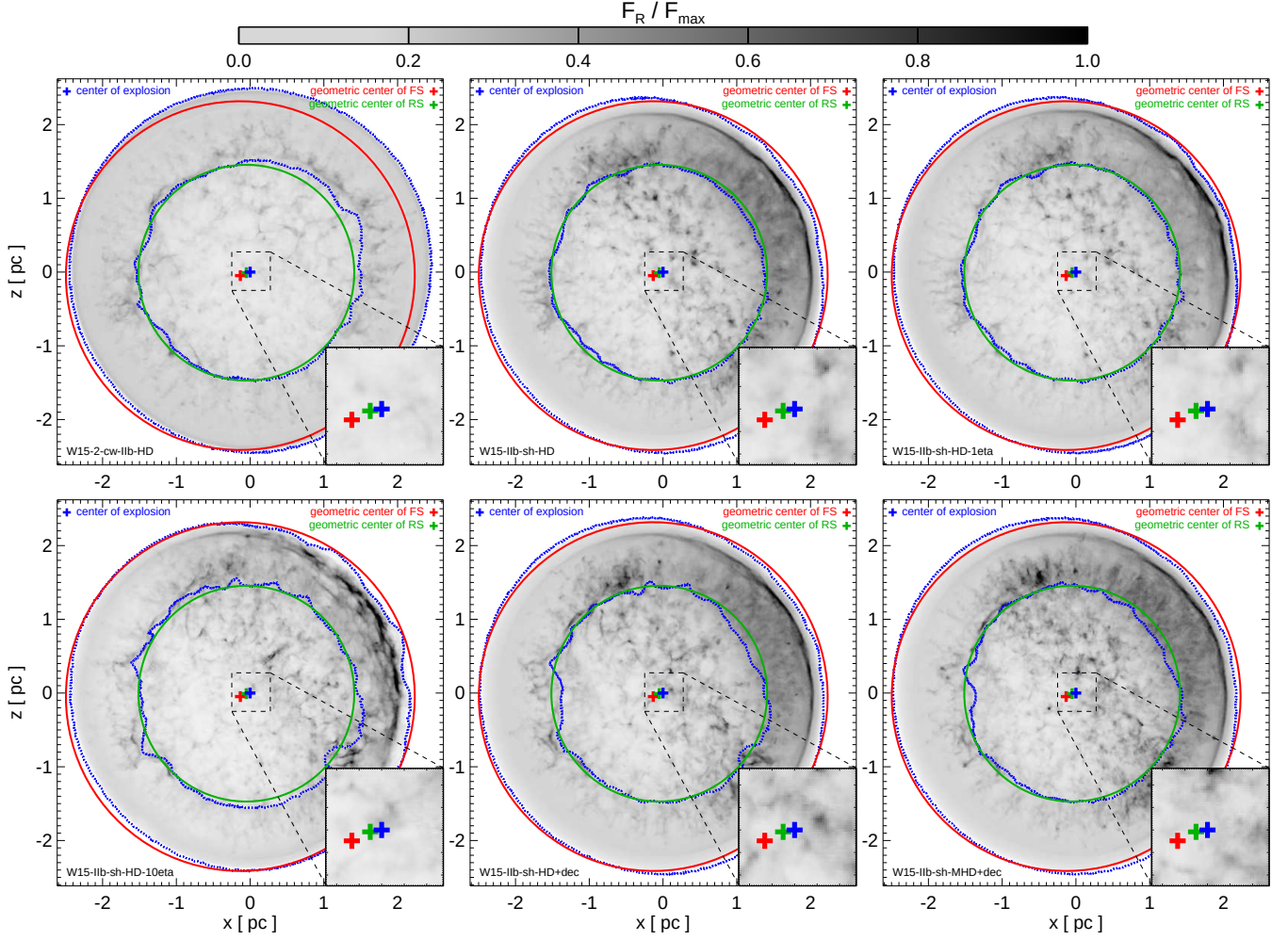
Fig. 8: Radio maps at the age of Cas A synthesized from the first six SNR models listed in Table 1, including model W15-2-cw-IIb-HD (presented in Paper I). The maps are normalized to the maximum radio flux, F_{\max} , in model W15-IIb-sh-HD-10eta. The blue dotted contours show cuts of the forward and reverse shocks in the plane of the sky passing through the center of the explosion (marked with a blue cross in each panel). The red and green circles mark the same cuts but for spheres roughly delineating the forward and reverse shocks, respectively, in models describing the remnant-shell interaction (the circles are the same in all the panels); the center of these spheres are marked with a cross of the same color (red or green) in each panel. These crosses represent the geometric center of the forward and reverse shocks, respectively, offset to the SE from the center of the explosion. The inset in the lower right corner of each panel is a zoom of the center of the domain.
