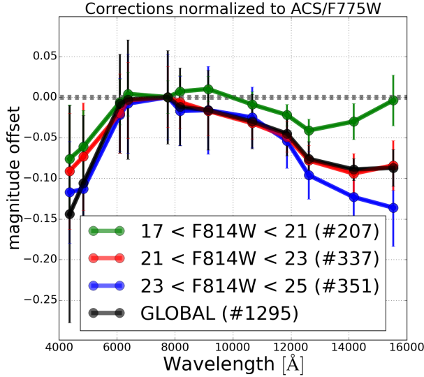
Figure 17. Magnitude corrections for the HST data (II). The same as in Figure 16 but dividing the sample in three magnitude bins: 17 < F814W < 21 (green), 21 < F814W < 23 (red) and 23 < F814W < 25 (blue). As before, it is observed a systematic trend with wavelength showing a clear spread in magnitude where fainter galaxies depart more from models.
