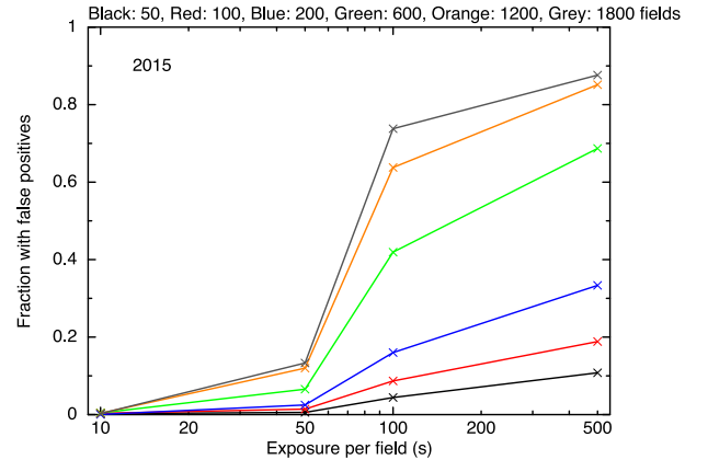
Figure 6. The fraction of simulations in which a source unrelated to the GW trigger was classified as a potential afterglow, because its measured flux was above the RASS limit due to Poisson noise. The data shown here are for the 2015 simulations, with galaxy targeting.
