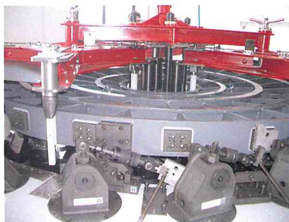
Fig. 13 – Primary mirror handling procedure (3/4): the mirror rests on the axial supports, lateral fixed points and supports are connected.
