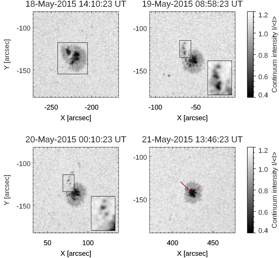
Figure 1. SHARP continuum images of AR NOAA 12348 acquired by HMI/SDO. The box in the top left panel indicates the IBIS FOV reported in Figures 6, 8, and 11. In the bottom right panel the red and blue boxes indicate the areas where the evolution of the parameters reported in Figure 9 were measured, while the red segment indicates the radial cut where the continuum intensity variation reported in the top left panel of Figure 10 has been computed. The animation of this figure begins on 2015 May 18 at 13:58:23 UT and ends on 2015 May 21 at 13:46:23 UT. The real-time duration of the animation is 72 s. Section 3.1 contains a description of the animation.
