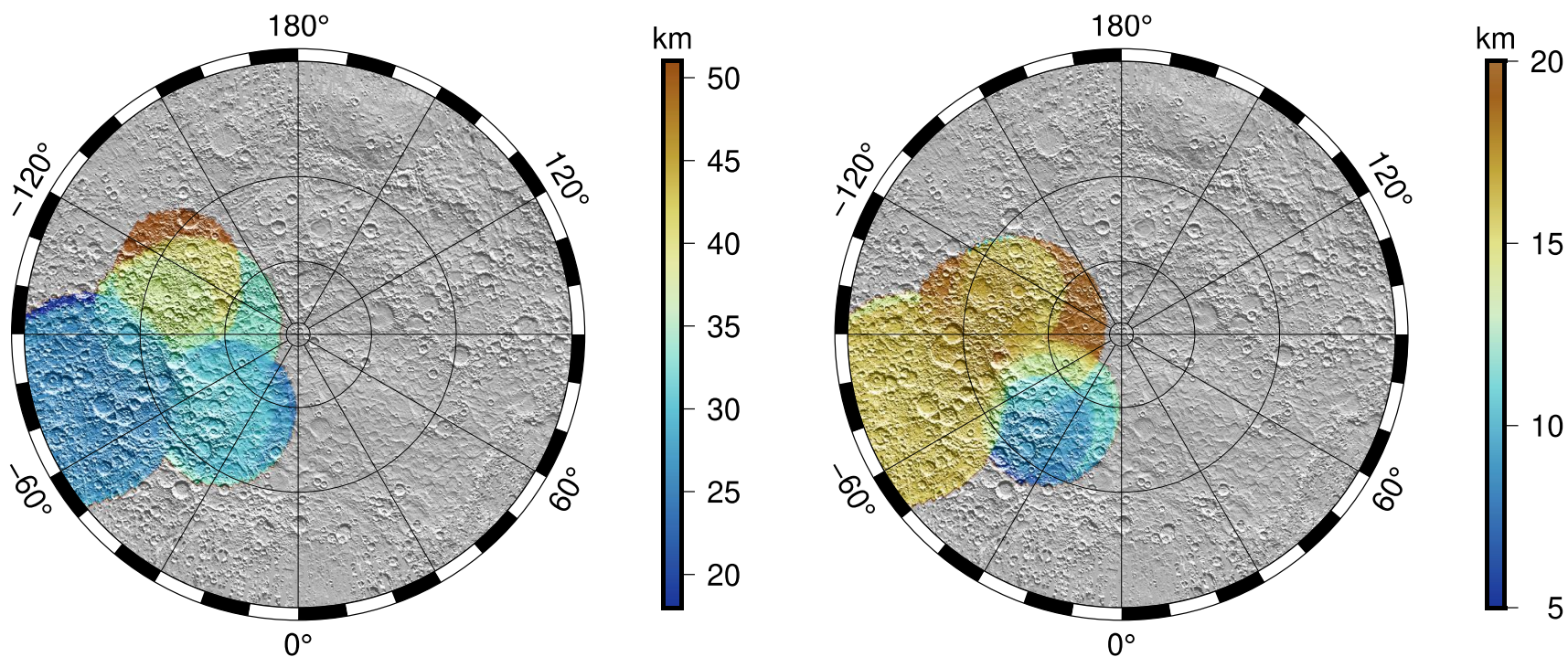
Figure S24 Maps of the lateral variations of the (left) crustal thickness and (right) its uncertainty in a polar stereographic projection from 30°N-latitude. This map is obtained by assuming surface loads only. Grey colors show regions where the localized admittance spectra do not allow to constrain the crustal density.
