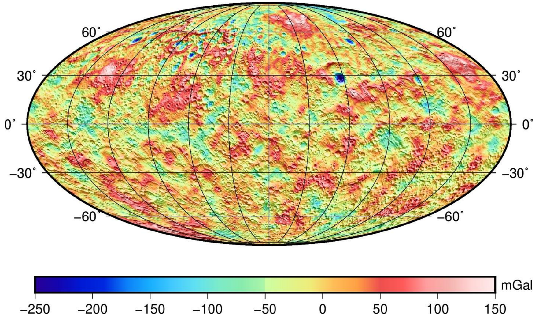
Figure S3 Global map of the free-air gravity anomaly (mGal) from our gravity solution retrieved by constraining the harmonic degrees greater than 10 with the power spectrum associated with gravity from topography [4] in a Mollweide projection centered on 0° longitude. These a priori formal uncertainties were computed by assuming a density crust of \rho_c = 2800 \text{ kg m}^{-3} .
