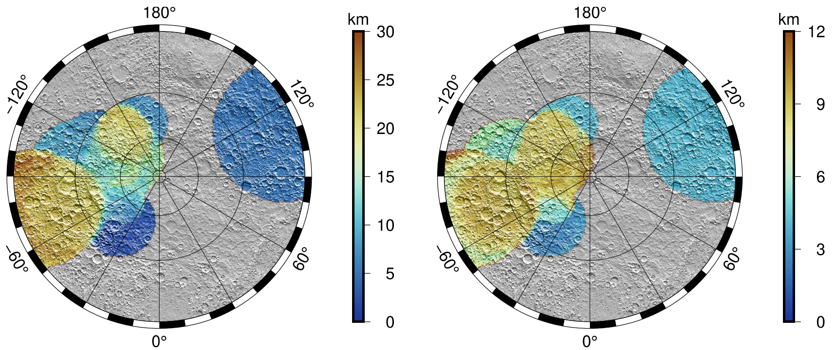
Figure S25 Maps of the lateral variations of the (left) elastic thickness and (right) its uncertainty in a polar stereographic projection from 30°N-latitude. This map is obtained by assuming surface loads only. Grey colors show regions where the localized admittance spectra do not allow to constrain the crustal density.
