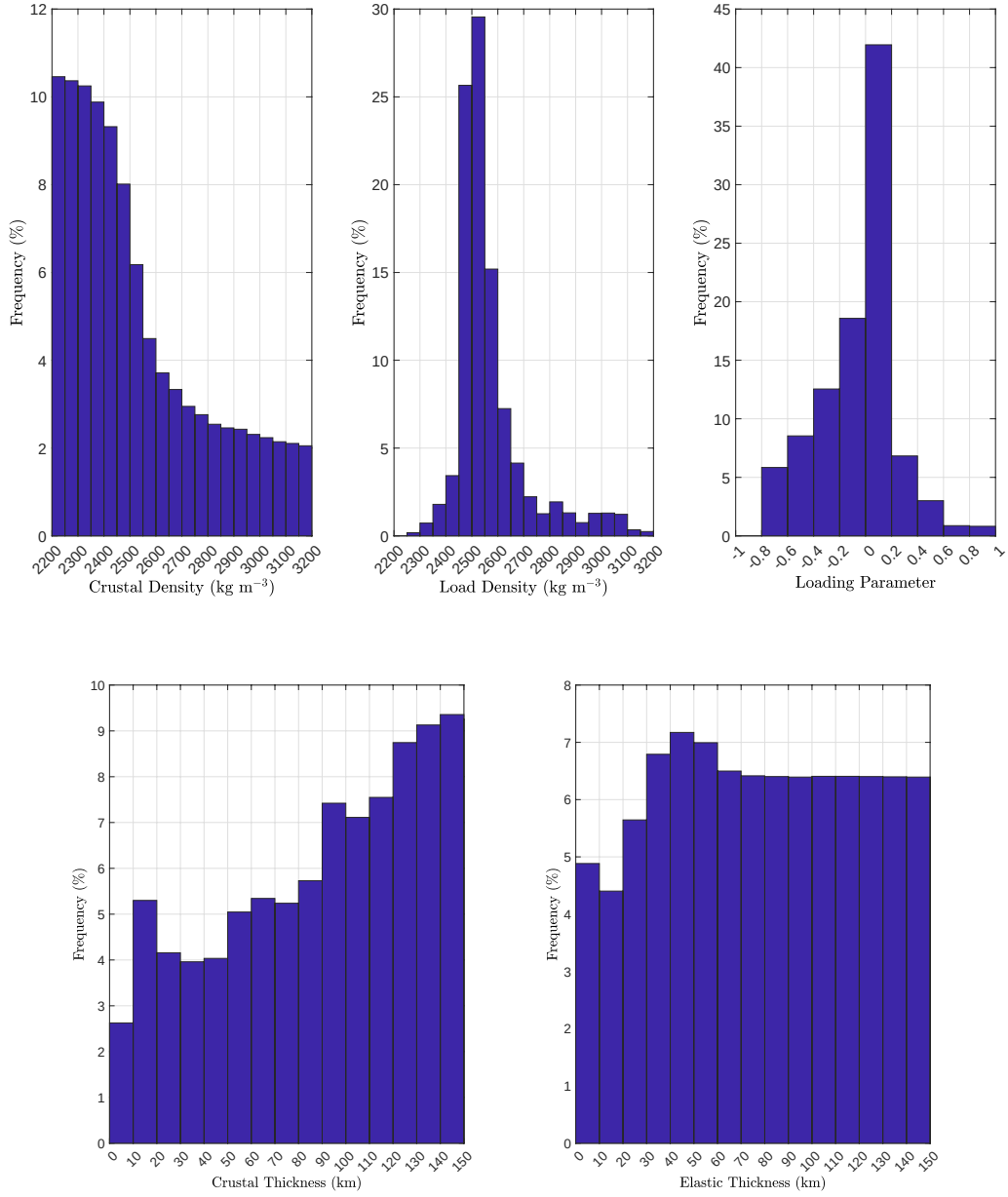
Figure S21 Histograms for the parameters of interest that are estimated through the admittance analysis of gravity and topography localized on the spherical cap described in the caption of Fig. 5. The predicted admittance spectrum is based on the top loads modeling as discussed in Sec. 4. The estimates of these parameters are: \rho_c = 2652 \pm 290 \text{ kg m}^{-3} ; \rho_l = 2542 \pm 125 \text{ kg m}^{-3} ; L = -0.26 \pm 0.31 ; T_c = 98 \pm 41 \text{ km} ; and T_e = 77 \pm 45 \text{ km} .
