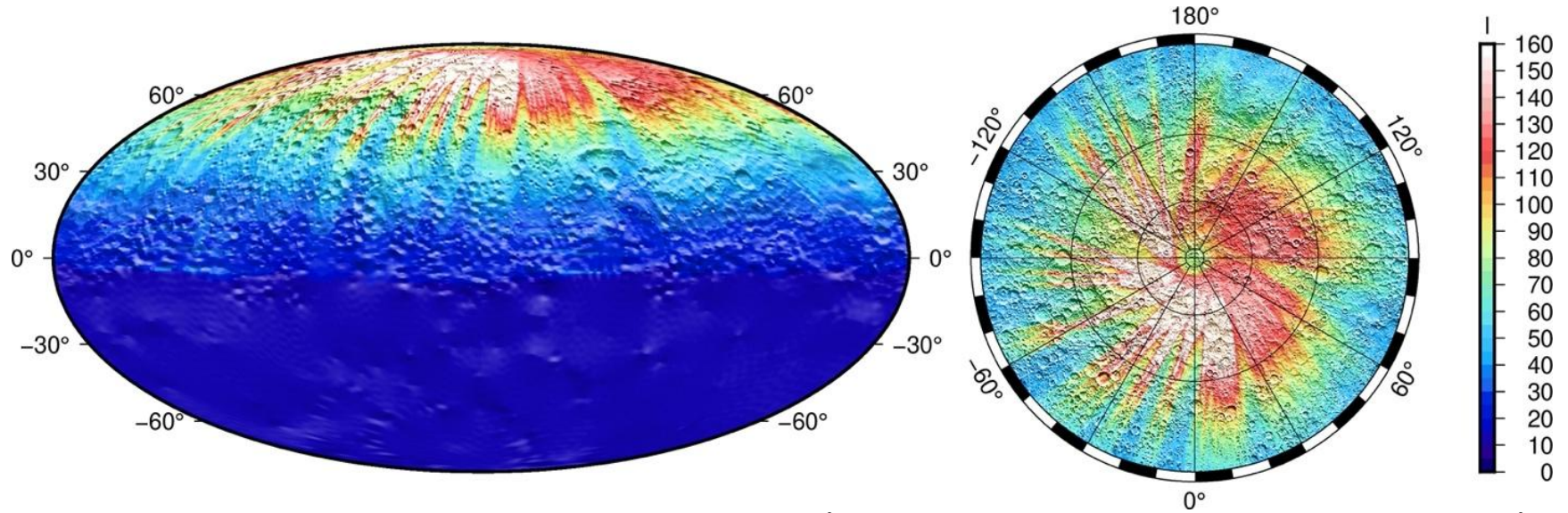
Figure S1 Degree strength map ( left ) in a Mollweide projection centered on 0° longitude and ( right ) in a polar stereographic projection from 30° N-latitude. This map was retrieved by comparing the expected acceleration profiles based on the Kaula power rule C_l = \frac{10 \times 10^{-5}}{l^2} (see Eq. 2) and the formal errors of the covariance matrix of our unconstrained gravity solution (see Eq. 1 in the paper by [3]).
