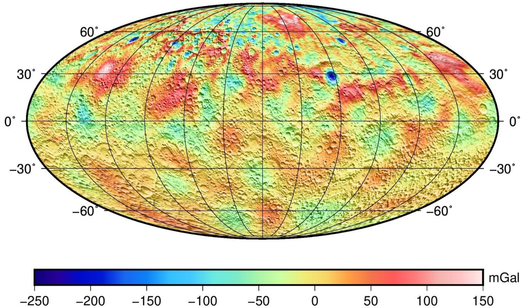
Figure S2 Global map of the free-air gravity anomaly (mGal) from the gravity field retrieved by constraining the measured acceleration profiles with the degree strength technique [3] in a Mollweide projection centered on 0° longitude. The shaded topographic relief in this figure and figures S3 and S4 is based on the U.S. Geological Survey (USGS) map by [4].
