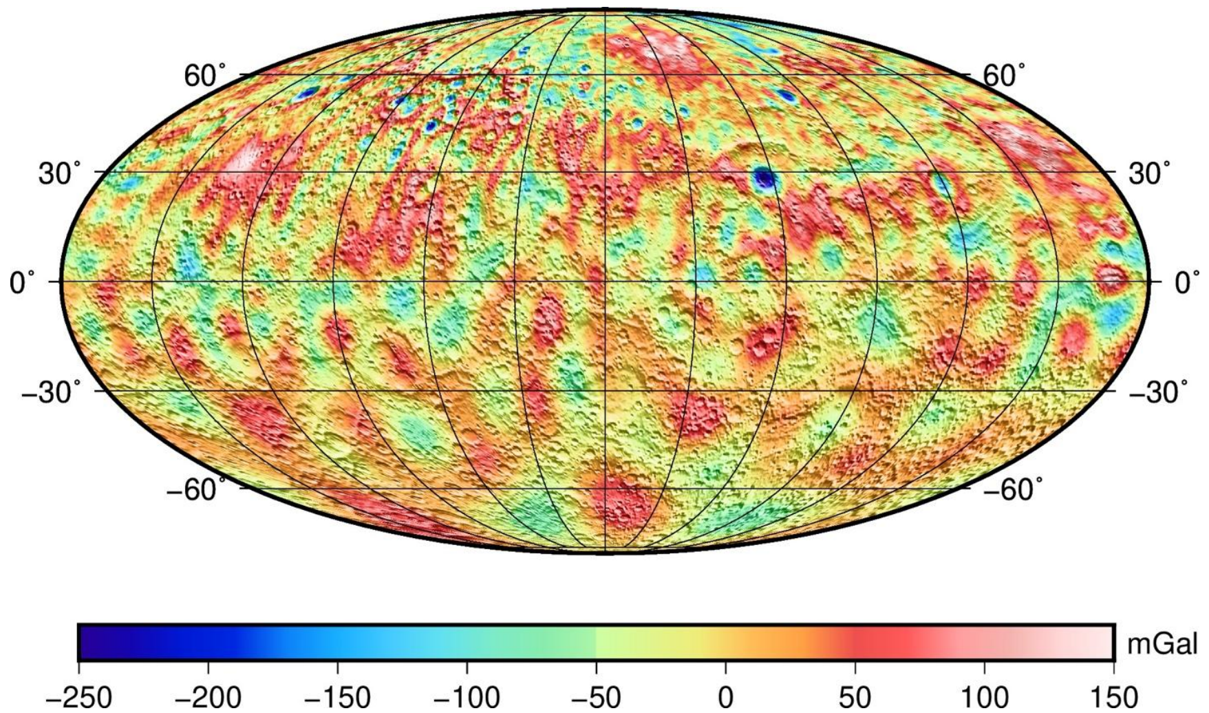
Figure S4 Global map of the free-air gravity anomaly (mGal) from gravity field HgM009 in a Mollweide projection centered on 0° longitude. The shaded topographic relief is based on the (USGS) map by [4].
