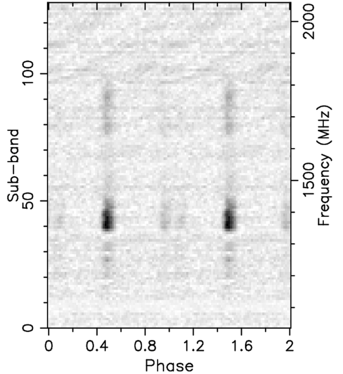
Fig. 10. Intensity as a function of pulse phase (x-axis) and frequency (y-axis) for the SRT observation performed in the L band on 19 August, 2019. Signal strength is not constant at all frequencies. At \sim 1.4 GHz there is a peak of intensity, while below 1.3 GHz and over 1.8 GHz the pulsed signal is almost absent.
