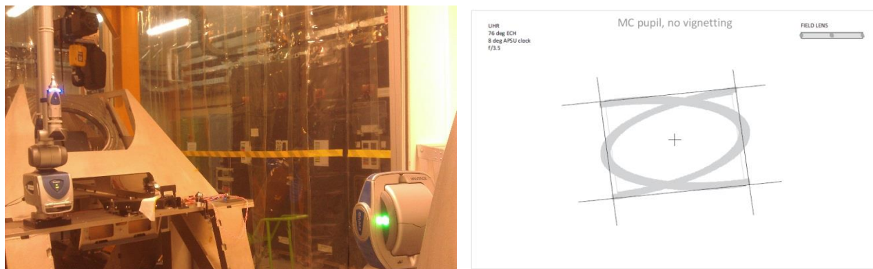
Figure 9: the laser tracker and the articulated arm mounted on the optical bench in the CCL at Paranal (left). The MC mask (right).
