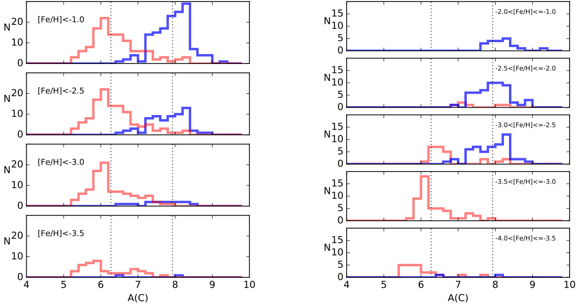
Figure 2. Left panel: Cumulative histograms of A(C) for the CEMP- s/rs stars (blue) and CEMP-no stars (red), in cuts of decreasing metallicity. Right panel: Differential histograms of A(C) for both sub-classes in intervals of declining metallicities. The dotted black lines represent the estimated location of the high-C and low-C peaks based on a two-component Gaussian fit (see text).
