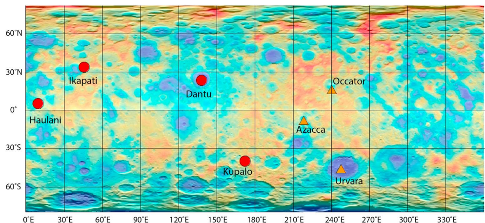
Figure 1. Global distribution of pitted crater materials on Ceres. Pitted materials similar to those identified in Vestan and Martian impact craters [Denevi et al. , 2012; Tornabene et al. , 2012] have been identified in Ikapati, Haulani, Dantu, and Kupalo craters (red circles) on Ceres. Depressions in Urvara, Occator, and Azacca may be degraded pits (orange triangles).
