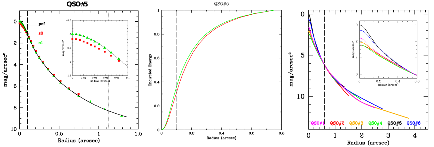
Figure 2. Left: comparison among the radial brightness profiles of the two stars (green triangles and red squares) used for the PSF fit (black solid line) for QSO#5. The dashed and dotted lines represent, respectively, the inner radius and maximum radius used for the PSF fit. Middle: encircled energy distribution of the two QSO#5 stars. Right: comparison of the radial brightness profile of the PSF for the six observed fields (solid color lines). The PSFs are very similar at radii larger than 0.6 arcsec, while they differ significantly in the inner core (see inset) due to different observing conditions and AO correction (see text). The dashed line indicates the radius at which all PSFs are normalized.
