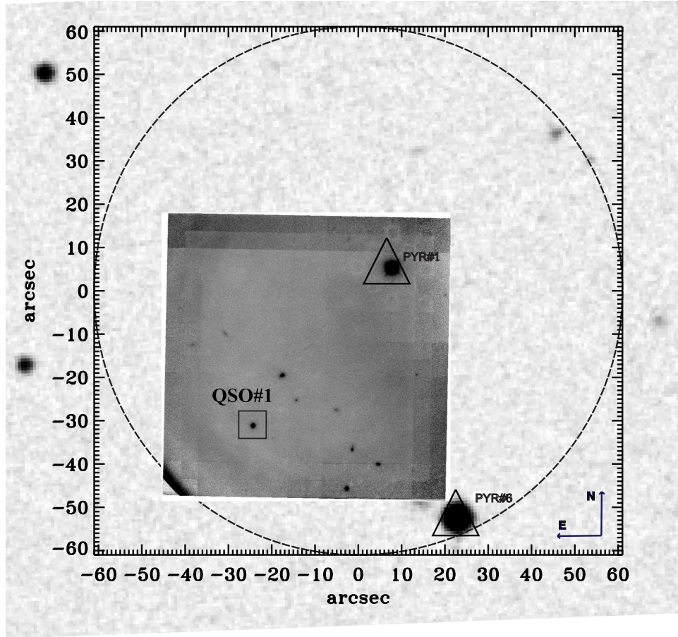
Figure 1. The 2 arcmin FOV for QSO#1 (DSS R filter image). The inner panel is the MAD (CAMCAO) final combined image in the K s filter. The two open triangles show the reference guide stars used ( V = 12.3 and 13.4 for Pyr 1 and Pyr 6, respectively). The open box indicates the QSO.
