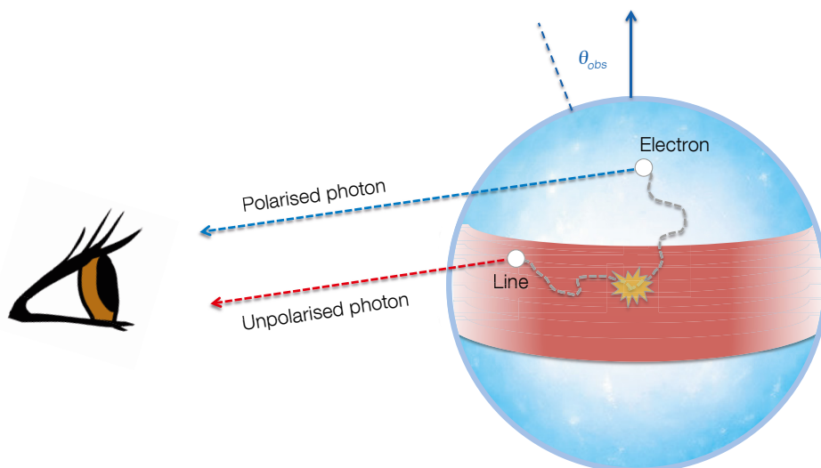
Figure 1. A cartoon illustrating the origin of polarisation in kilonovae. Photons escaping the ejected material from the red component are preferentially depolarised by line interactions, while those leaving the ejecta from the blue component are more likely to be polarised by electron scattering. These both contribute to the total polarisation signal that could be observed in future kilonova events.
