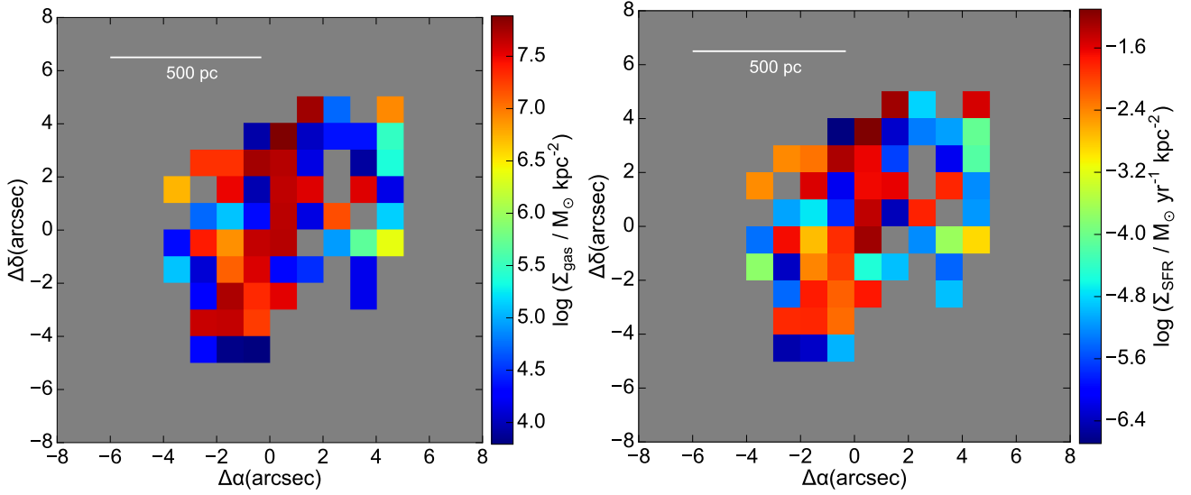
Figure 16. Gas mass surface density ( \Sigma_{\text{gas}} , left panel) and Star Formation surface density ( \Sigma_{\text{SFR}} , right panel) for the galaxy IZw18.
