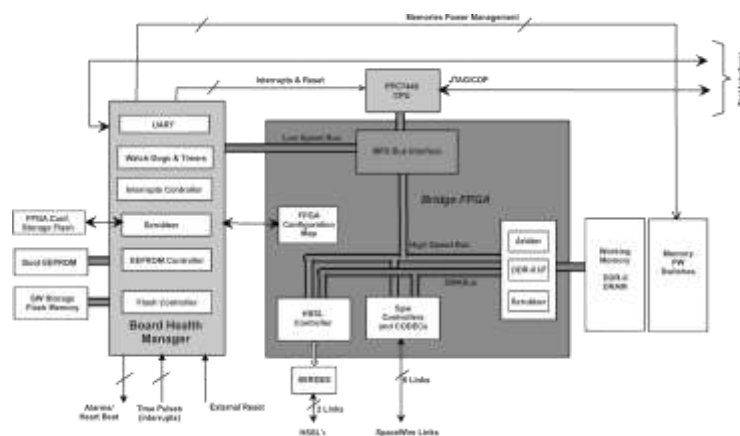
Fig. 1 The overall system Architecture
