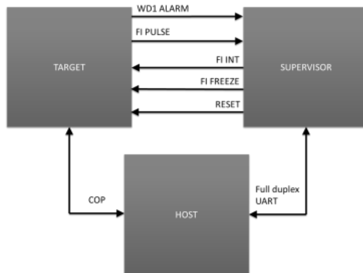
Fig. 2 Fault Injection System architecture
