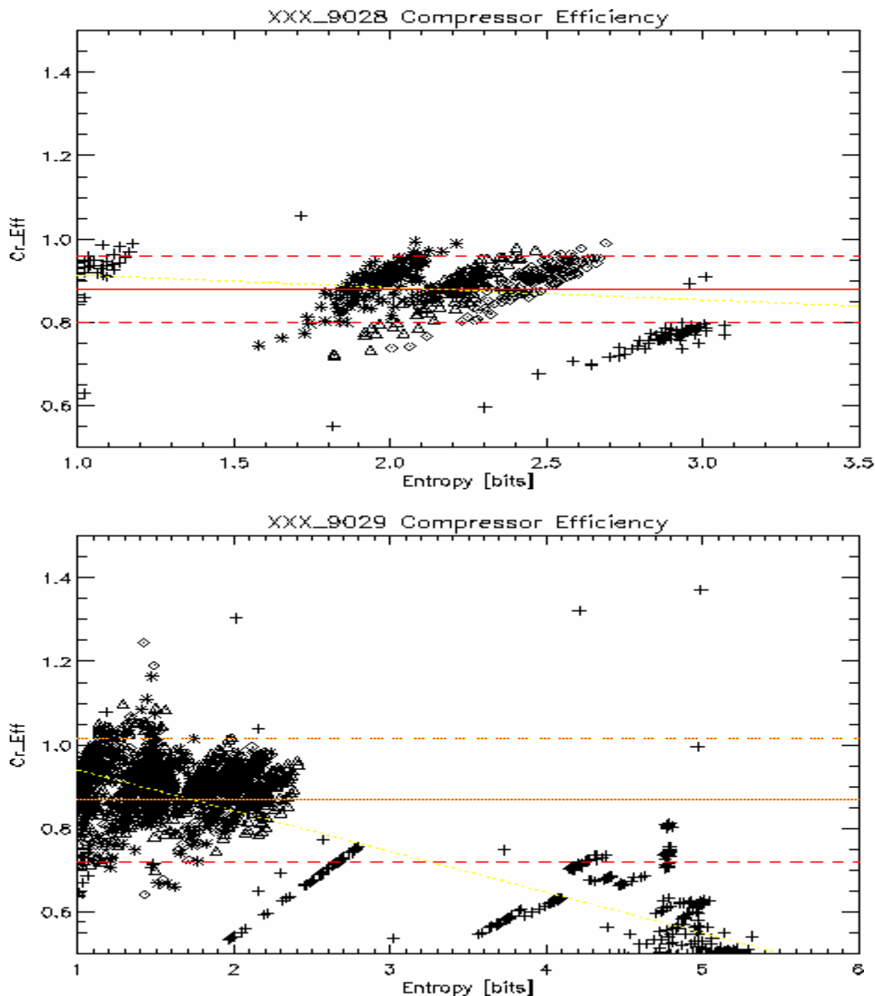
Fig A.4 Cr_Eff as a function of entropy for XXX_9028 (upper frame) and XXX_9029 (lower frame). Symbols as in Fig.A.2. Red horizontal line is the Averaged Cr_Eff, dashed horizontal lines
