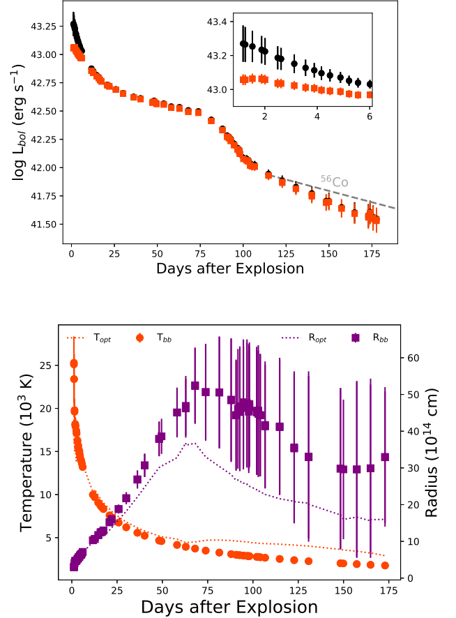
Figure 8. Top: Bolometric lightcurve integrated from NUV to NIR. Inset shows a zoom in of the first few days. The red points indicate the observed luminosity, while the black points come from blackbody corrections to the data. The ^{56}\text{Co} decay rate is indicated in gray. Bottom: Temperature and radius evolution of SN 2017gmr derived from the photometry. The temperature is plotted in red, and the radius in purple.
