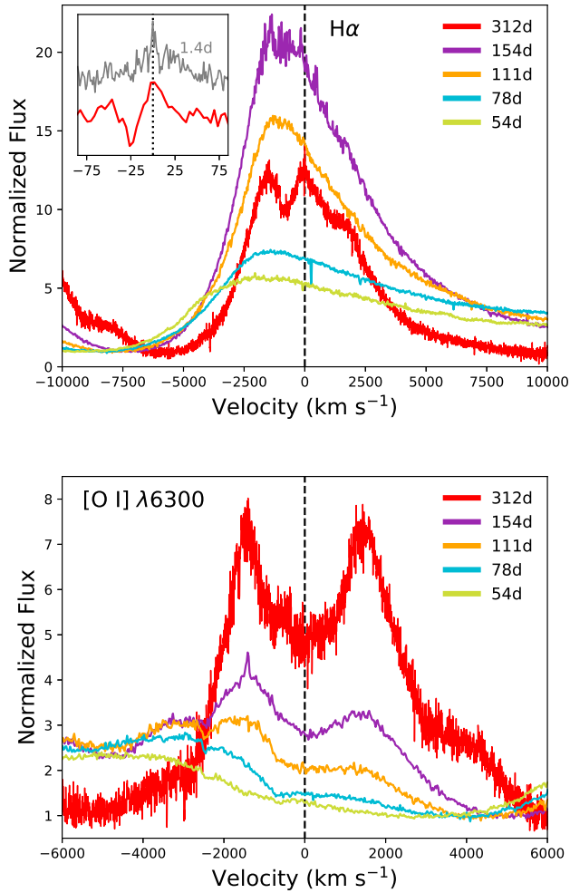
Figure 18. Evolution of the H \alpha (top) and [O I] \lambda\lambda 6300, 6363 Å (bottom) emission lines from our moderate and high-resolution spectra. The lines have been normalized to the minimum of the H \alpha P-Cygni line. The multi-peaked shape begins to arise between 110-150 days, but is clearly evident by our last spectrum on day 312.
