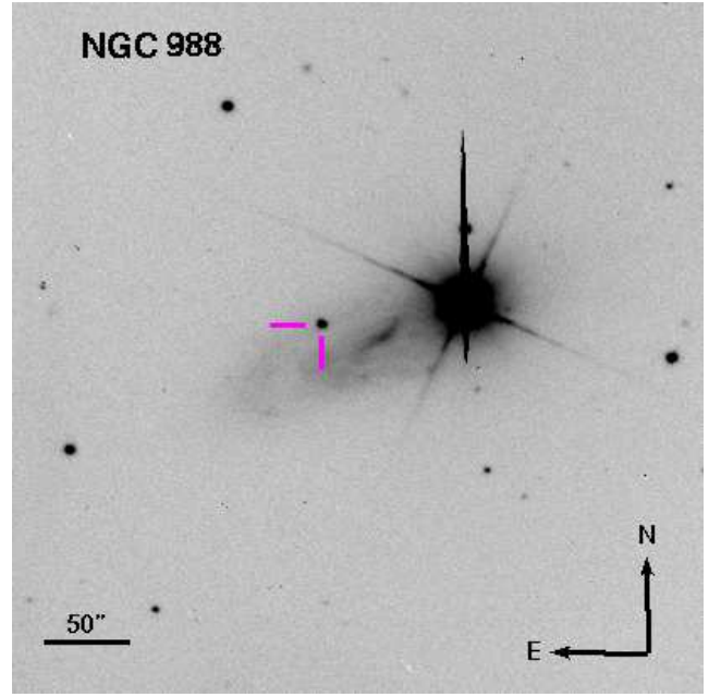
Figure 1. SN 2017gmr in NGC 988 taken on 2017 November 25 in V-band with Super-LOTIS. Image is 7' \times 7' .
