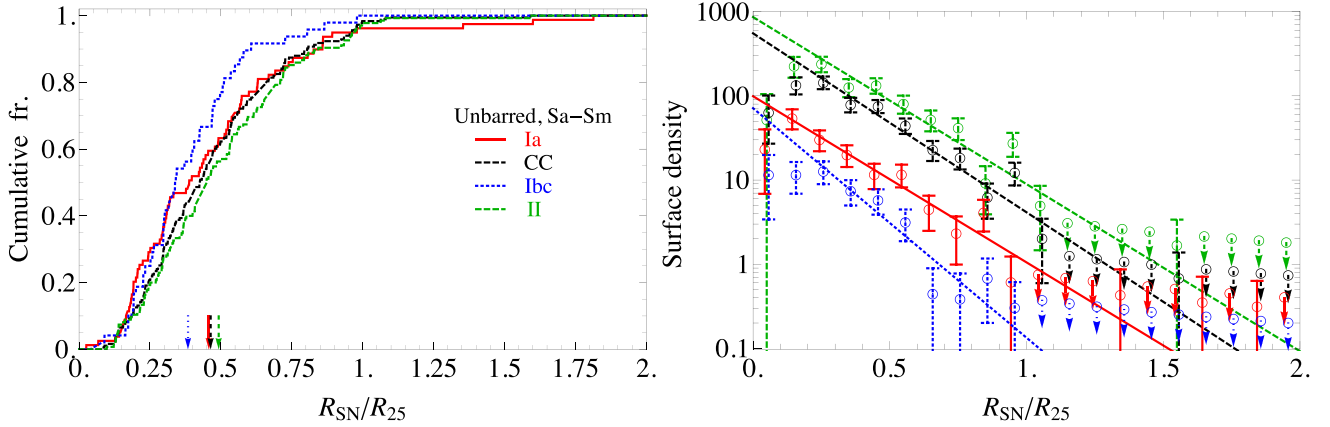
Figure 3. Left: cumulative fractions of the different types of SNe versus deprojected and normalized galactocentric radius ( \tilde{r} = R_{\text{SN}}/R_{25} ) in unbarred Sa–Sm host galaxies. The mean \tilde{r} values of each SNe type are shown by arrows. Right: surface density distributions (with arbitrary normalization) of the different types of SNe in the same subsample of hosts. The different lines show the maximum likelihood exponential surface density profiles estimated for the inner-truncated disc. The error bars assume a Poisson distribution. Down arrows represent the upper-limits of surface density (with \pm 1 SN if none is found). For better visibility, the distributions are shifted vertically sorted by increasing the mean \tilde{r} as one moves upwards.
