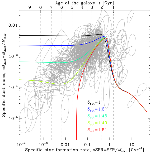
Fig. 15. Effect of outflow on the sM_{\text{dust}} – s\text{SFR} relation. The data are identical to panel c of Fig. 14. The colored lines represent our dust evolution model. We have fixed all the parameters close to their maximum a posteriori values, except the outflow rate, \delta_{\text{out}}: \tau_{\text{SFH}} = 0.8 \text{ Gyr} , \psi_0 = 40 M_{\odot} \text{ yr}^{-1} , \delta_{\text{in}} = 1.0 , \delta_{\text{SN}} = 0.01 , \epsilon_{\text{grow}} = 4500 , and m_{\text{gas}}^{\text{dest}} = 1200 M_{\odot}/\text{SN} . The different lines correspond to different values of \delta_{\text{out}} . The top axis displays the age of the galaxy corresponding to the particular SFH of the model run. We have used a Salpeter (1955) IMF.
