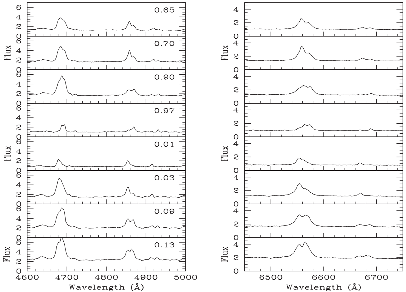
Figure 5. Sequence of spectra of He II and H \beta (left) and H \alpha (right) obtained on 2016 June 5 at peak of outburst. The fluxes are in units of 10^{-14} erg cm ^{-2} s ^{-1} Å ^{-1} . Phases are marked in the upper right of the left plots.
