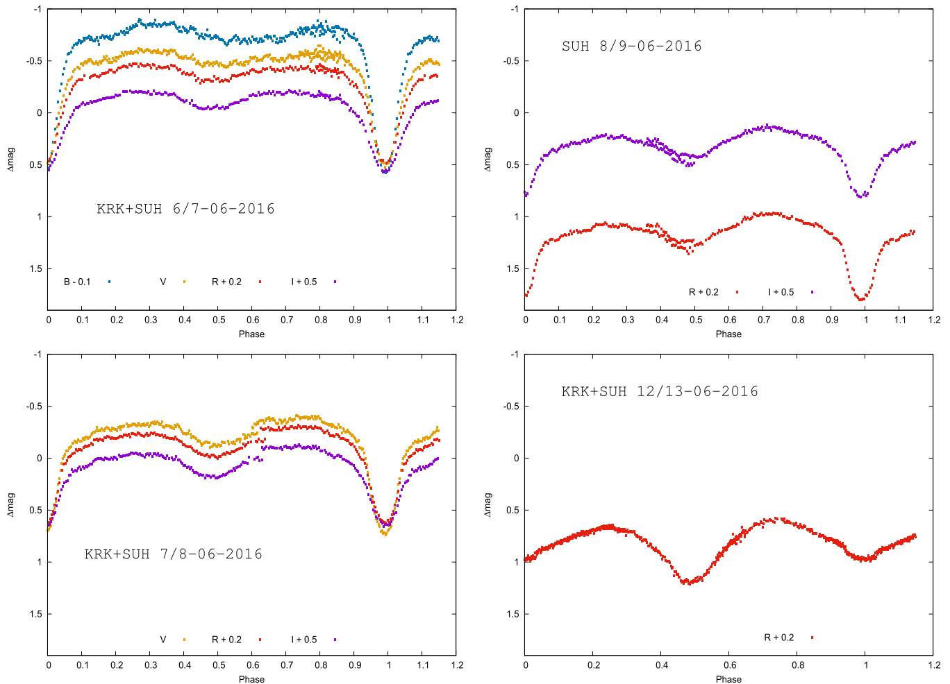
Figure 2. Multicolor light curves of J1621 at outburst. The scale of each panel is the same to show the decline in brightness and changing shape of the light curve. \Delta\text{mag} denotes the magnitude difference between J1621 and the comparison star (3UC269-134839).
