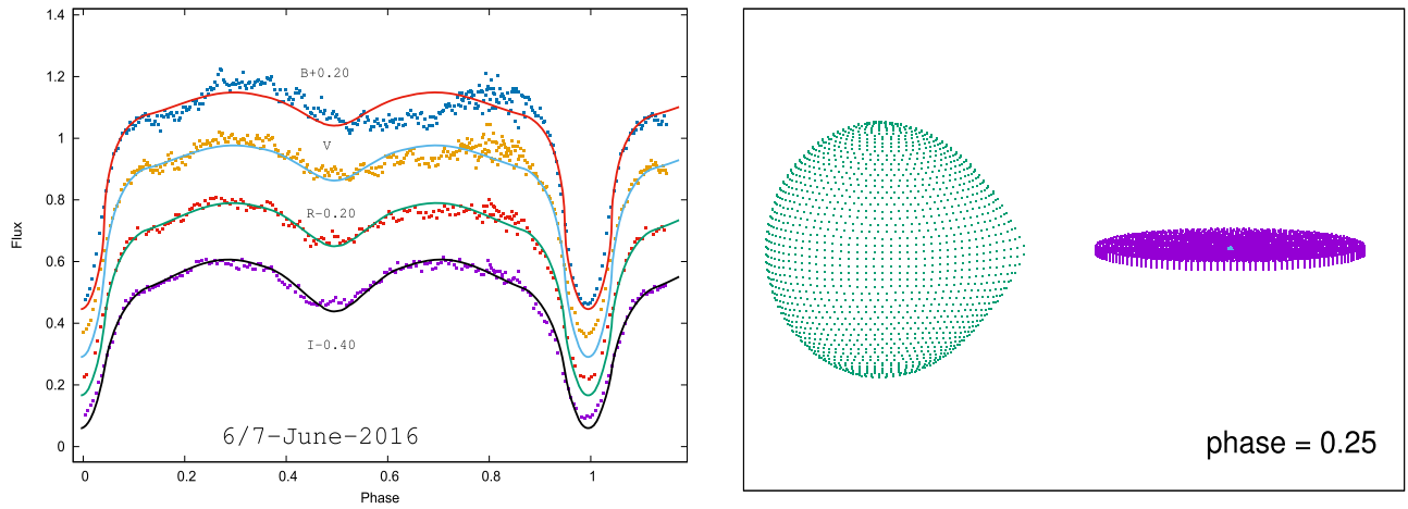
Figure 10. Best fit to observations at outburst obtained within the circular disk model (left) and a view of the J1621 model at phase 0.25 (right panel).
