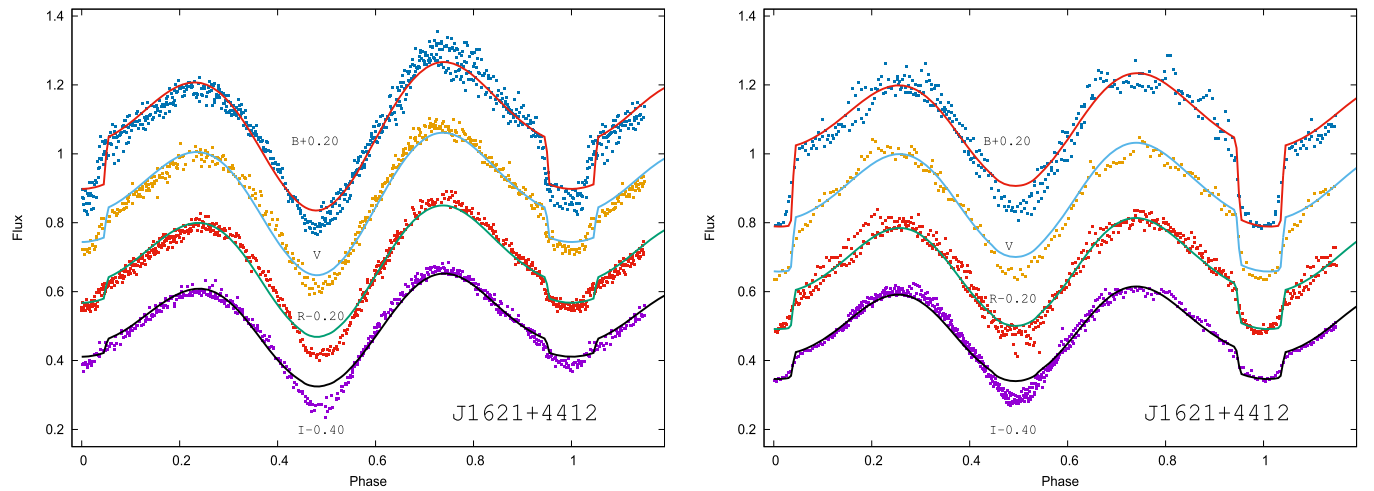
Figure 8. Best fit obtained within the W-D model (IPB = 0 only). The left panel shows data taken in 2016 August, while the right panel shows data taken in 2017 March. Observations are plotted by dots, while continuous lines represent the model.
