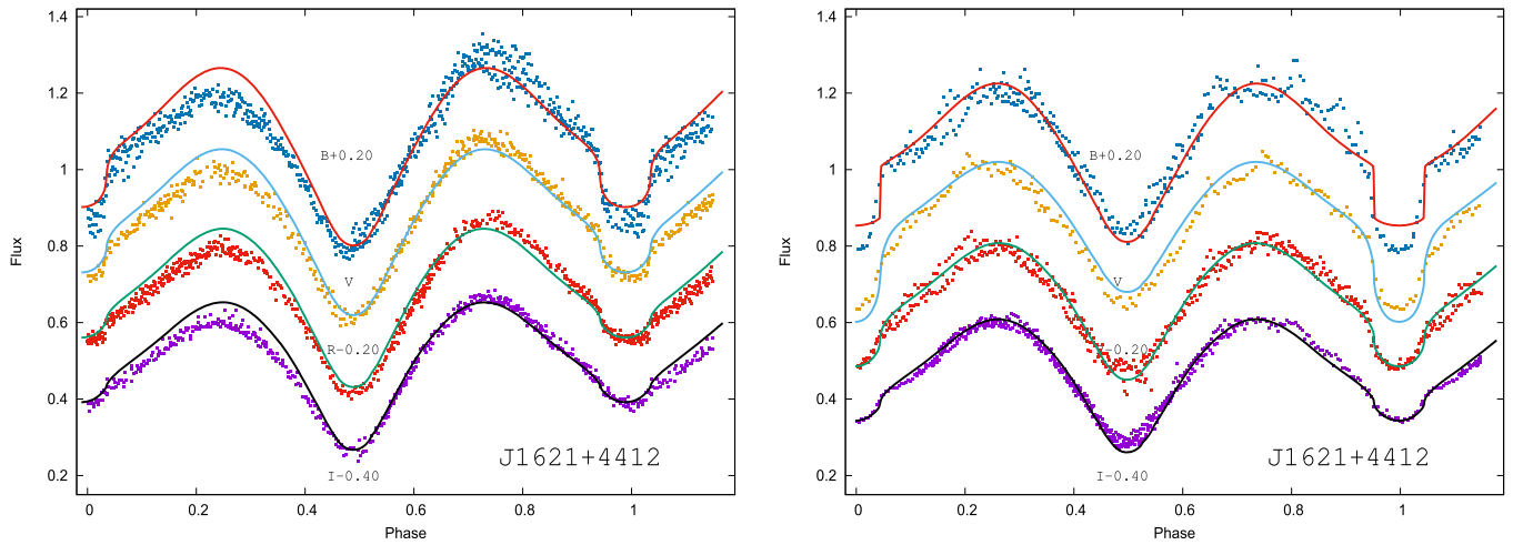
Figure 9. Best fit obtained within the circular disk model (top left) for the mass ratio fixed at q = 0.45 . The observed points between phase 0.15 and 0.4 were discarded in computations (see the text for an explanation).
