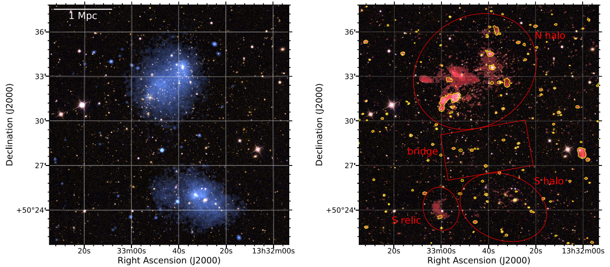
Figure 1. Composite images of A1758 obtained from the superposition of an optical SDSS g, r, i mosaic with Chandra (blue) and with a LOFAR image at 144 MHz with a resolution of 7.6 \text{ arcsec} \times 5.4 \text{ arcsec} (red) and a rms noise of 60 \mu\text{Jy beam}^{-1} . Yellow and red regions indicate the mask used to subtract discrete sources and the regions adopted to measure the flux densities in the low-resolution images, respectively.
