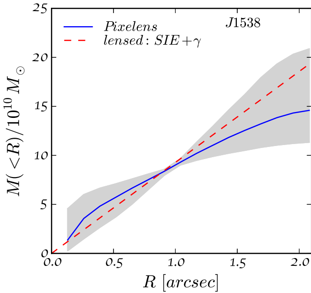
Figure 5. Comparison of the enclosed mass profiles reconstructed by PIXELEN and LENSED for the lens J1538+5817. The blue solid line indicates the PIXELEN ensemble median with 90 percent confidence interval (shaded area). The red dashed line shows a Singular Isothermal Ellipsoid (SIE) model plus shear.
