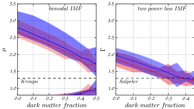
Figure 11. IMF parameters versus dark matter fraction ( f_{\text{DM}} ). an increase in the DM fraction causes the \alpha -interval to shrink and the IMF parameter interval, defined by the intersection of (1 - f_{\text{DM}}) \times M_{\text{tot}} and M_* to shift. Median (solid line) and 68 per cent confidence intervals (shaded region) are shown for the whole set of lenses. Red (blue) colour denotes H -band (I, V-band) data. The left-hand panel shows the results for a bimodal IMF parametrization, hence the two separate \mu -intervals. The right-hand panel shows the two-segment power-law parametrization, which constrains \Gamma only from one side.
