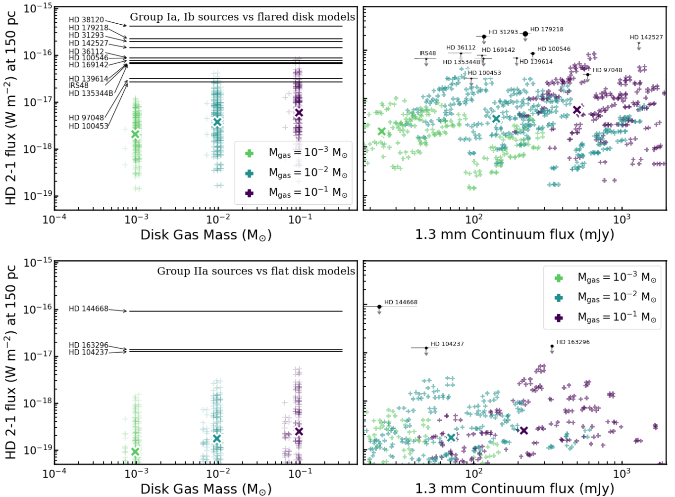
Fig. B.1. Upper limits on HD 56\mu\text{m} line flux for the sample of Herbig Ae/Be disc systems (black lines) compared with our grid of DALI disc models (crosses). The top panels show the group I sources compared to models with flaring angle \psi = 0.3 . The bottom panels show the group II sources compared to models with \psi = 0.0 . Left: models are separated based on gas mass. Right: HD 2–1 upper limits set against 1.3 mm continuum fluxes for both observations and models.
