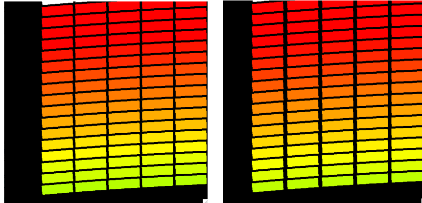
Figure 23. A detail of the OPD map for a MM near the innermost radius of ATHENA. Left: constant rib thickness. Right: variable rib thickness with the lateral coordinate. The MM parameter values 7 are: f = 12 m, R_0 = 277 mm, N = 34 , L_0 = 110 mm, h = 0.6 mm, \tau = 0.14 mm, w = 2.1 mm, t = 0.17 mm at the center rib and (in the right graph) increasing by 0.013 mm/pore from the central ribs toward the plate edges.
