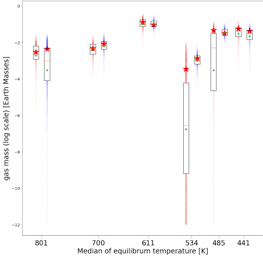
Extended Data Fig. 6 Gas mass fraction of the HD 110067 planets as a function of their equilibrium temperature. We infer two values per planet by assuming the different planetary masses from our METHOD I (red) and METHOD II (blue) radial velocity analyses. The boxes, orange lines, green triangles, and red stars represent respectively the 25% and 75% percentiles, medians, means, and modes of the posterior distributions. The opacity of the vertical lines is proportional to the posterior distribution.
