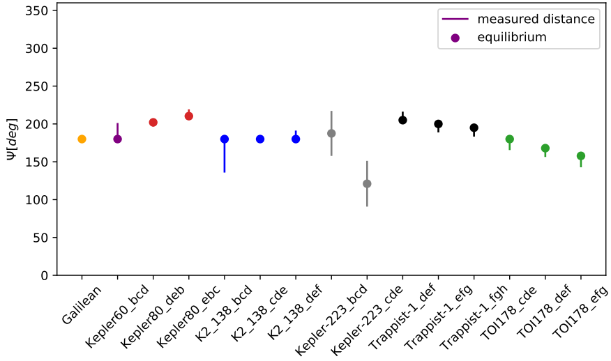
Extended Data Fig. 2 Generalized three-body Laplace angles for known systems in resonant chains. Included are the Galilean satellites, Kepler-60 [12, 115], Kepler-80 [159], K2-138 [112], Kepler-223 [110], TRAPPIST-1 [13], and TOI-178 [10]. Measurements belonging to the same system are marked with the same color. The line marks the observed distance to the theorized equilibrium (marked with a circle). The distances are estimated at 0th order in eccentricity [110, 111]. For most systems, a single estimation of the generalized Laplace angle is made, while [110] made an estimation for each Kepler quarter.
