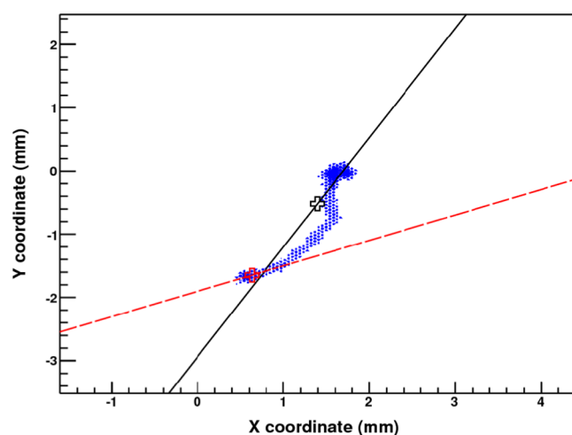
Fig. 4 Example of a photoelectron track produced by the absorption of a photon at 22 keV acquired with the GPD filled with an Ar (70%)–DME (30%) gas mixture at the pressure of 2 bar. The upper black cross is the barycenter of the charge distribution and the black solid line is the main axis of the track. The lower red cross is the absorption point and the red dashed line is the emission direction of the photoelectron.
