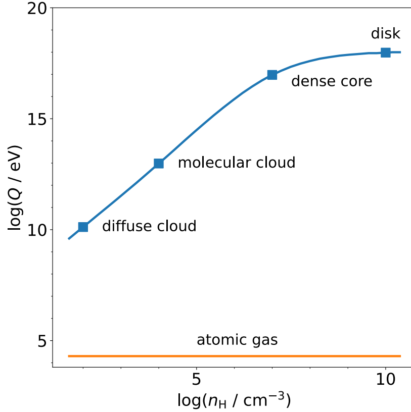
FIGURE 1.1 Average heat input Q per CR ionization as a function of the total H density n_H (adapted from Glassgold et al. 2012). Bottom curve, Q_{\text{at}} ; top curve, Q_{\text{mol}} .
