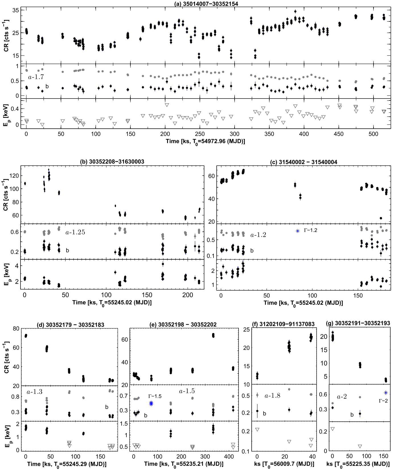
Figure 7. Most densely sampled 0.3–10 keV light curves with brightness doubling/halving in 2009–2012.
