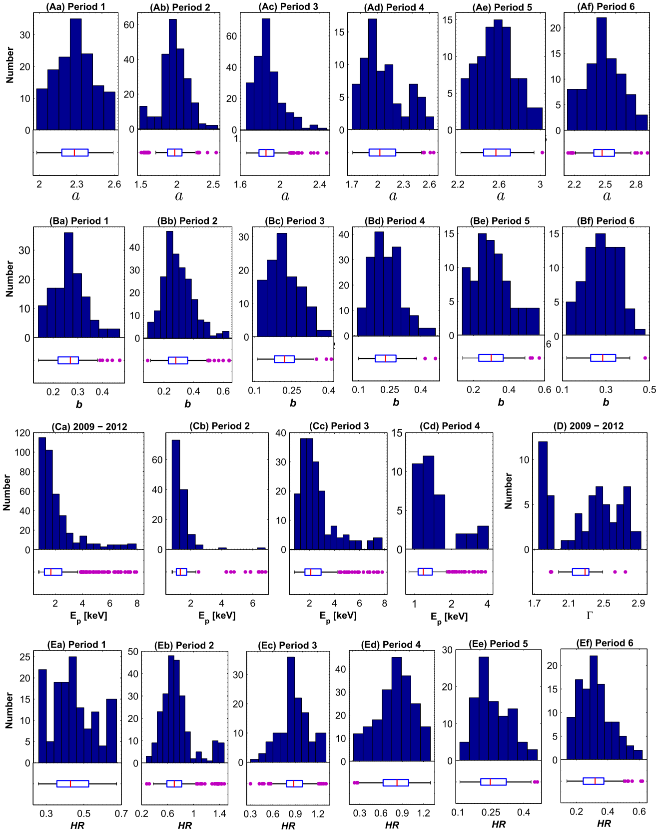
Figure 1. Distribution of the spectral parameter values in different periods. The red line within each box-plot corresponds to the median of the distribution, and the purple points represent the outliers.
