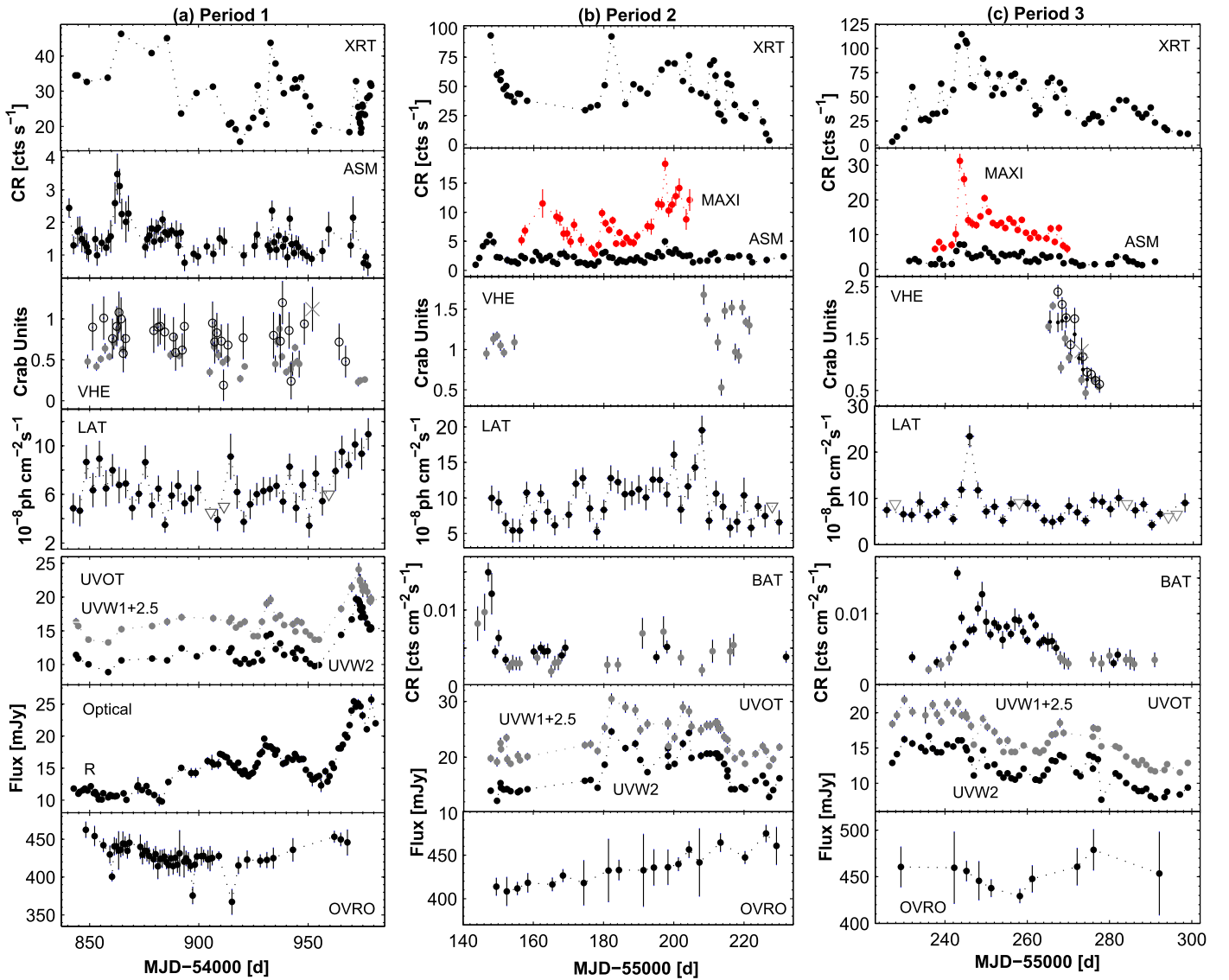
Figure 4. MWL variability of Mrk 421 in different periods during 2009–2012. The daily bins are used for the XRT, FACT, UVOT, Steward, 15 GHz, and light curves and the two-day bins for the LAT data. The radio-band observations were performed with the 40 m OVRO telescope (Richards et al. 2011), and the corresponding data are retrieved from http://www.astro.caltech.edu/ovroblazars/ . In the VHE light curves, black points correspond to the VERITAS data, and the gray points, circles, and asterisks correspond to those from the MAGIC, Whipple, and HAGR observations, respectively. The triangles in the LAT-related plots stand for the 2\sigma upper limits to the 0.3–300 GeV flux when the source was detected below the 3\sigma significance. The BAT detections of Mrk 421 with 5\sigma and 3\sigma significances are shown with black and gray points, respectively (see the next page for Figures 4(d)–(f)).
