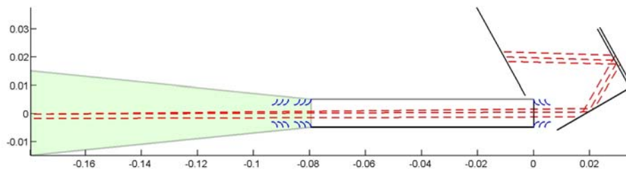
Figure 3.1. Examples of particle trajectories (red dashed lines) inside SCENARIO, for ~1 keV ENAs
