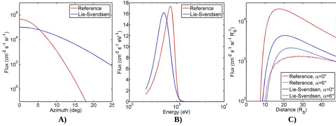
Figure 1.4. Differential flux ( \text{cm}^{-2} \text{s}^{-1} \text{sr}^{-1} ) versus azimuthal direction along the ecliptic plane, with 0^\circ towards the Sun (panel A) and differential flux per unit energy versus energy (panel B) for the two slow solar wind models. Panel C: differential flux ( \text{cm}^{-2} \text{s}^{-1} \text{sr}^{-1} R_S^{-1} ) versus distance for the slow solar wind reference model and the Lie-Svendsen model for different azimuthal angles indicated in the boxes.
