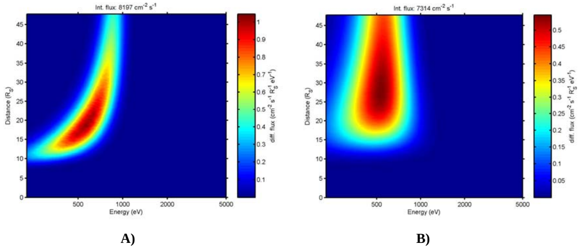
Figure 1.5. Contour plot of the differential flux per unit distance and energy at 48 R_S as a function of energy and distance for the slow solar wind reference (panel A) and Lie-Svendsen (panel B) models. The flux is integrated over all directions.
